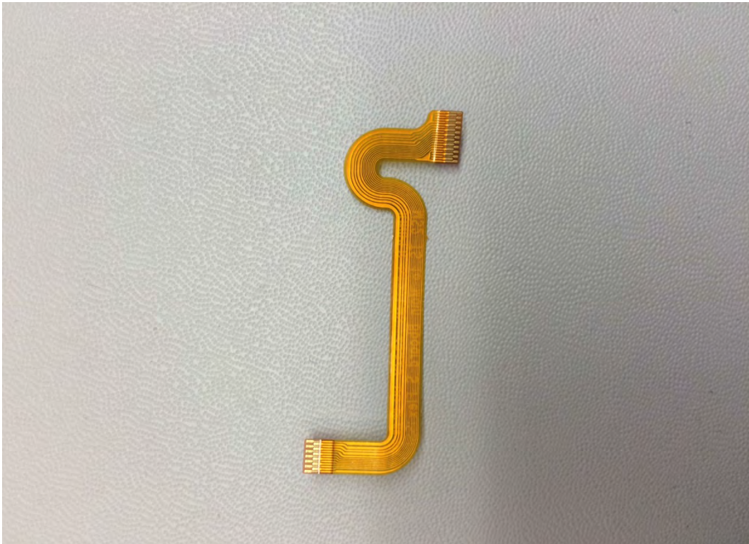
MS2 "S" connector flex (back)
