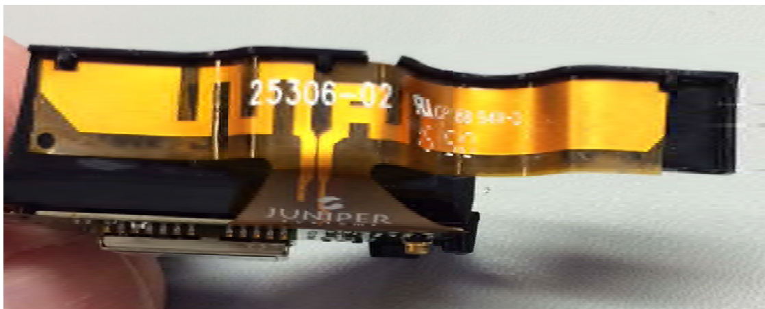
MS2 GNSS flex (back)
