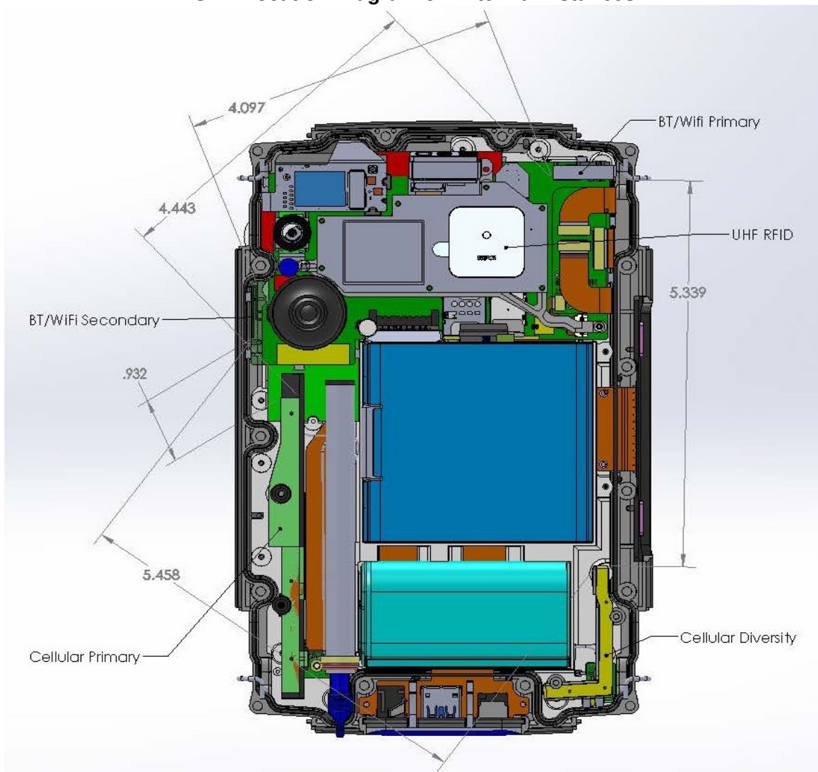
Figure 9.1 SAR Location Diagram of Antenna Distances
