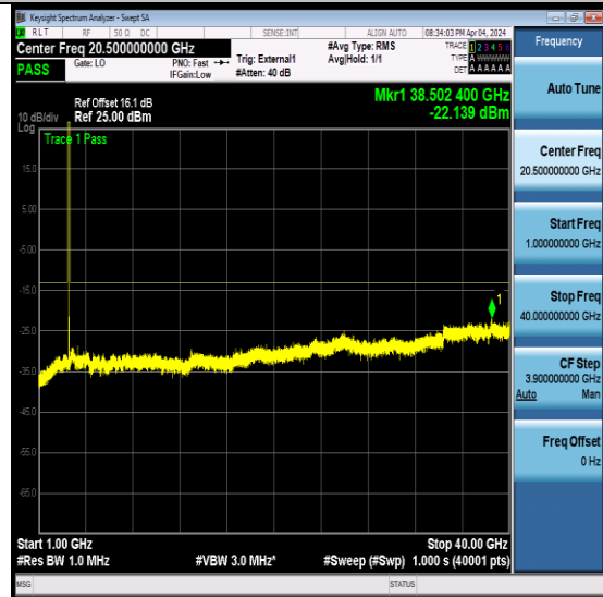
NTNV-N78-3450-3550-PC2-30-60-M-CP-QPSK- Edge_1RB_Left-Ant1-PASS
