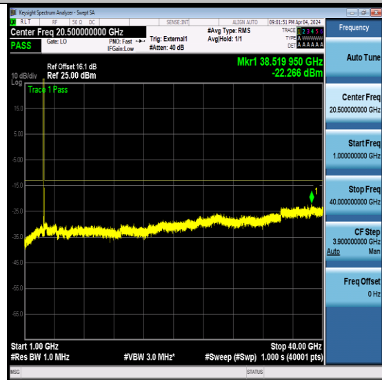
NTNV-N78-3450-3550-PC2-30-60-H-CP-QPSK- Edge_1RB_Left-Ant7-PASS
