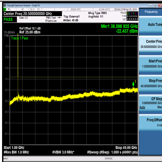
NTNV-N78-3450-3550-PC2-30-20-H-CP-QPSK- Edge_1RB_Left-Ant1-PASS
