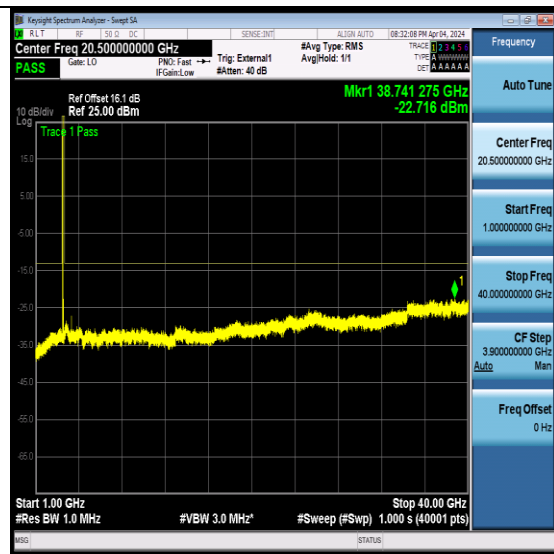
NTNV-N78-3450-3550-PC2-30-60-L-CP-QPSK- Edge_1RB_Left-Ant1-PASS
