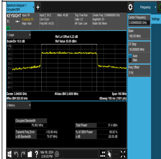
NTNV-N77-3700-3980-PC2-30-80-M-DFT- 16QAM-Outer_Full-Ant1-PASS
