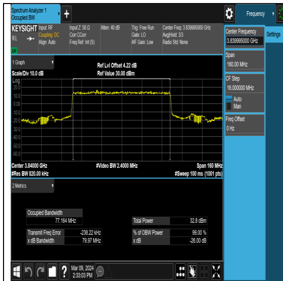
NTNV-N77-3700-3980-PC2-30-80-M-DFT- P12BPSK-Outer_Full-Ant1-PASS
