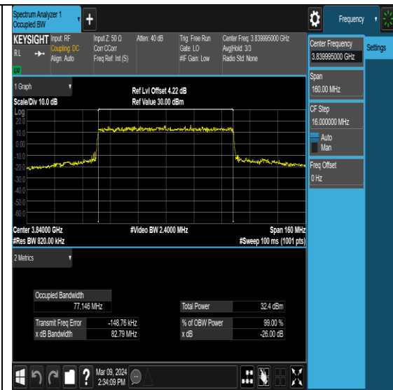
NTNV-N77-3700-3980-PC2-30-80-M-DFT-QPSK- Outer_Full-Ant1-PASS
