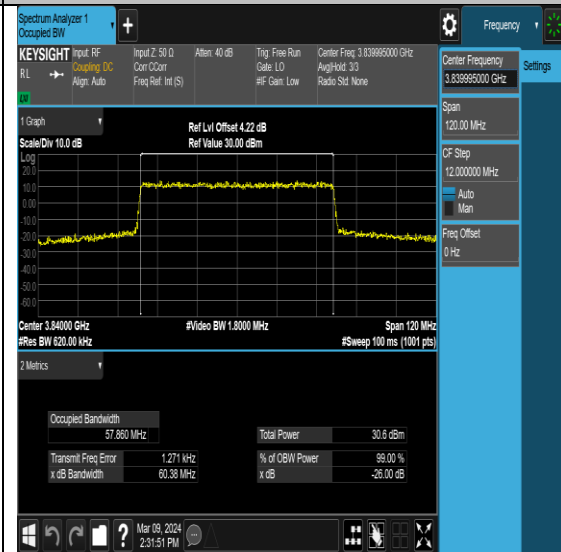
NTNV-N77-3700-3980-PC2-30-60-M-DFT-256QAM-Outer_Full-Ant1-PASS
