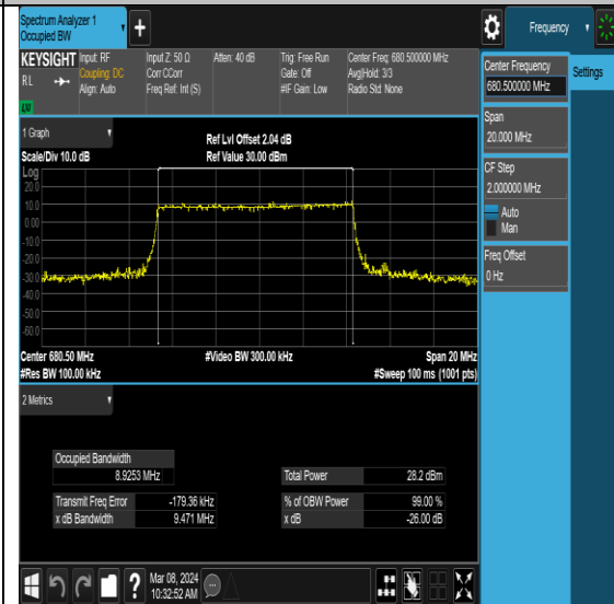
NTNV-N71-PC3-15-10-M-DFT-16QAM-Outer_Full-Ant0-PASS
