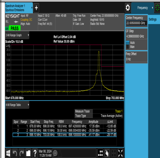
NTNV-N71-PC3-15-20-H-DFT-QPSK-Edge_1RB_Right-Ant0-PASS
