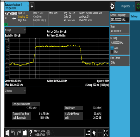
NTNV-N71-PC3-15-20-M-DFT-PI2BPSK-Outer_Full-Ant0-PASS
