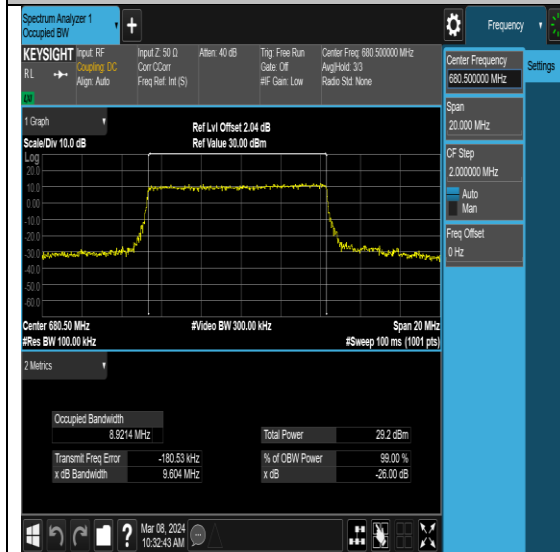
NTNV-N71-PC3-15-10-M-DFT-QPSK-Outer_Full-Ant0-PASS
