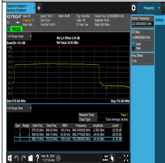
NTNV-N71-PC3-15-20-H-DFT-QPSK-Outter_Full-Ant0-PASS
