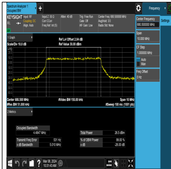
NTNV-N71-PC3-15-5-M-DFT-256QAM-Outer_Full-Ant0-PASS
