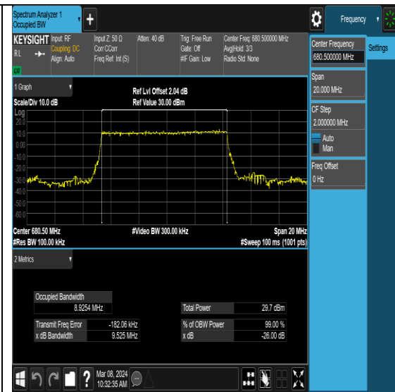
NTNV-N71-PC3-15-10-M-DFT-PI2BPSK-Outer_Full-Ant0-PASS
