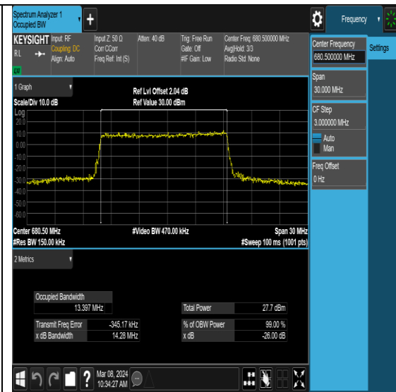
NTNV-N71-PC3-15-15-M-DFT-64QAM-Outer_Full-Ant0-PASS
