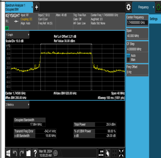
NTNV-N66-PC3-15-20-M-DFT-PI2BPSK-Outer_Full-Ant0-PASS
