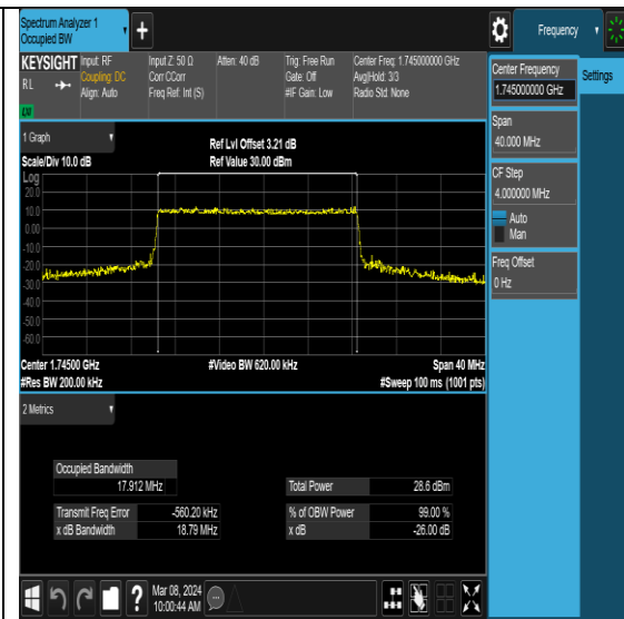
NTNV-N66-PC3-15-20-M-DFT-16QAM-Outer_Full-Ant0-PASS
