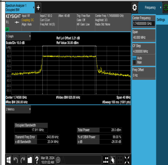
NTNV-N66-PC3-15-20-M-DFT-256QAM-Outer_Full-Ant0-PASS
