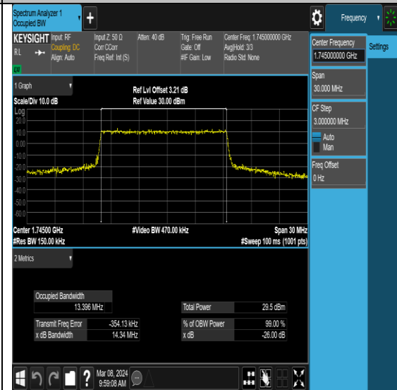
NTNV-N66-PC3-15-15-M-DFT-QPSK-Outer_Full-Ant0-PASS
