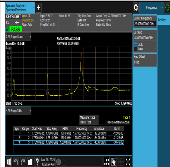
NTVN-N66-PC3-15-15-H-DFT-QPSK-Edge_1RB_Right-Ant0-PASS
