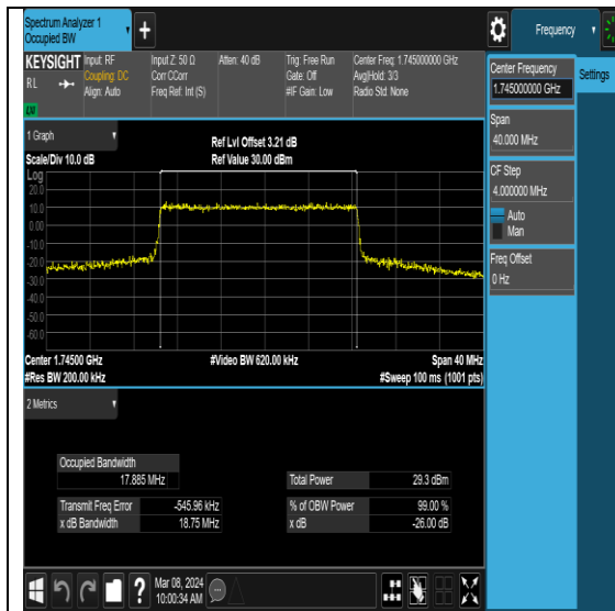
NTNV-N66-PC3-15-20-M-DFT-QPSK-Outer_Full-Ant0-PASS
