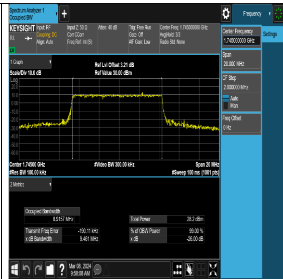
NTNV-N66-PC3-15-10-M-DFT-256QAM-Outer_Full-Ant0-PASS
