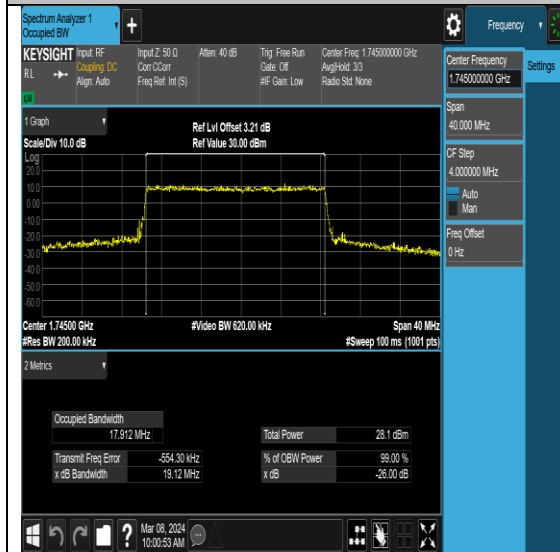
NTNV-N66-PC3-15-20-M-DFT-64QAM-Outer_Full-Ant0-PASS
