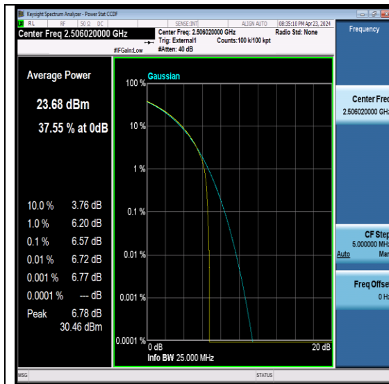
NTNV-N41-PC2-30-20-L-CP-QPSK-Outter_Full-PASS
