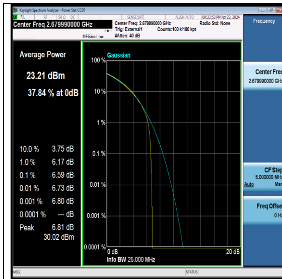
NTNV-N41-PC2-30-20-H-CP-QPSK-Outter_Full-PASS
