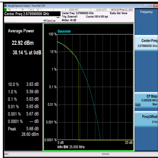
NTNV-N41-PC2-30-20-H-CP-QPSK-Edge_1RB_Left-PASS
