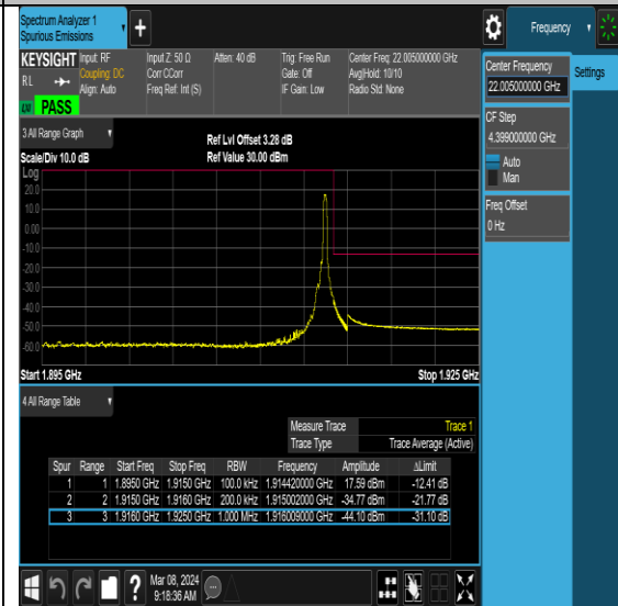
NTNV-N25-PC3-15-20-H-DFT-QPSK-Edge_1RB_Right-Ant0-PASS
