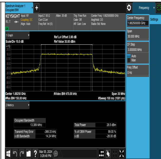
NTNV-N25-PC3-15-15-M-DFT-64QAM-Outer_Full-Ant0-PASS
