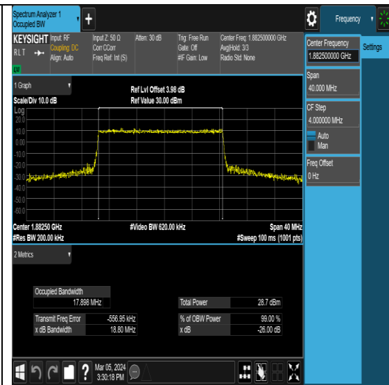
NTNV-N25-PC3-15-20-M-DFT-16QAM-Outer_Full-Ant0-PASS
