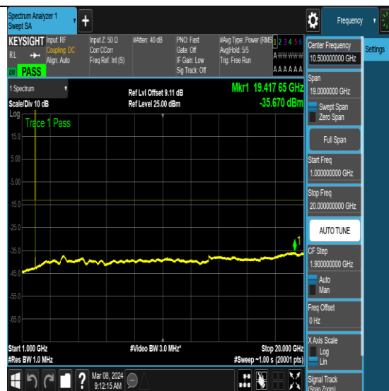
NTNV-N25-PC3-15-20-H-DFT-QPSK- Edge_1RB_Left-Ant0-PASS
