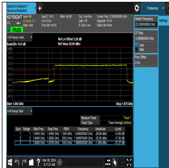
NTNV-N25-PC3-15-20-L-DFT-QPSK-Outter_Full-Ant0-PASS
