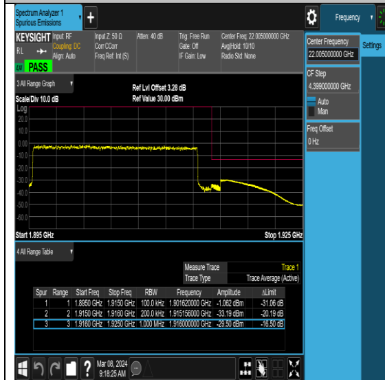
NTNV-N25-PC3-15-20-H-DFT-QPSK-Outter_Full-Ant0-PASS
