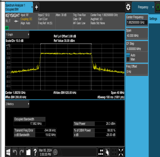
NTNV-N25-PC3-15-20-M-DFT-256QAM-Outer_Full-Ant0-PASS
