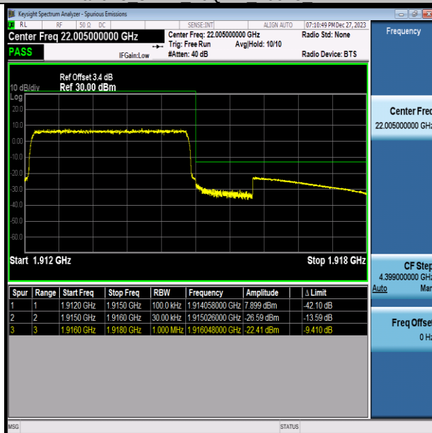
Band25 3MHz 16QAM 26675 15RB#0
