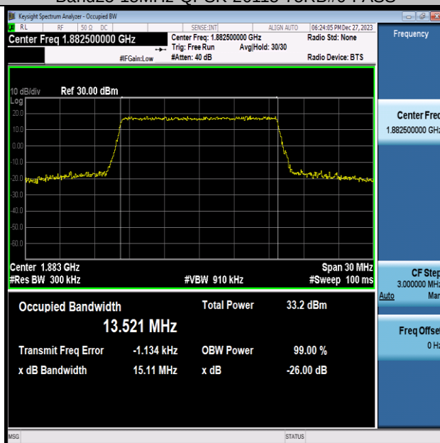
Band25-15MHz-QPSK-26365-75RB#0-PASS
