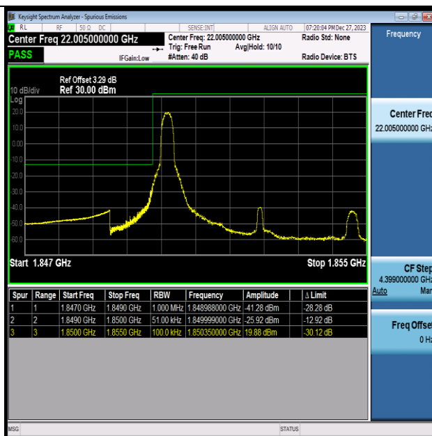
Band25 5MHz 16QAM 26065 1RB#0
