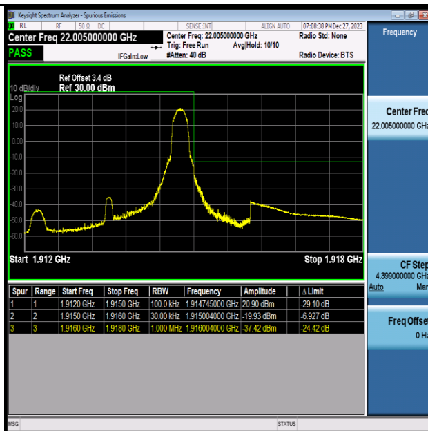
Band25 3MHz 16QAM 26675 1RB#14
