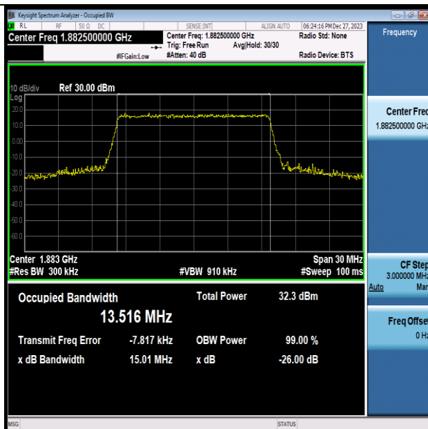
Band25-15MHz-16QAM-26365-75RB#0-PASS
