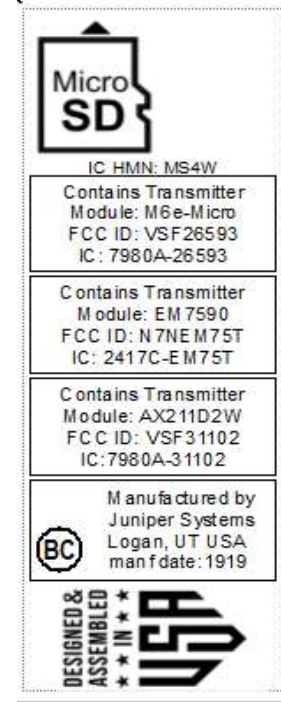
Bluetooth/Wi-Fi Radio, cellular Radio, and Micro RFID Radio
