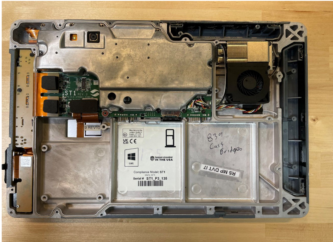
Internal photo with mainboard shield
