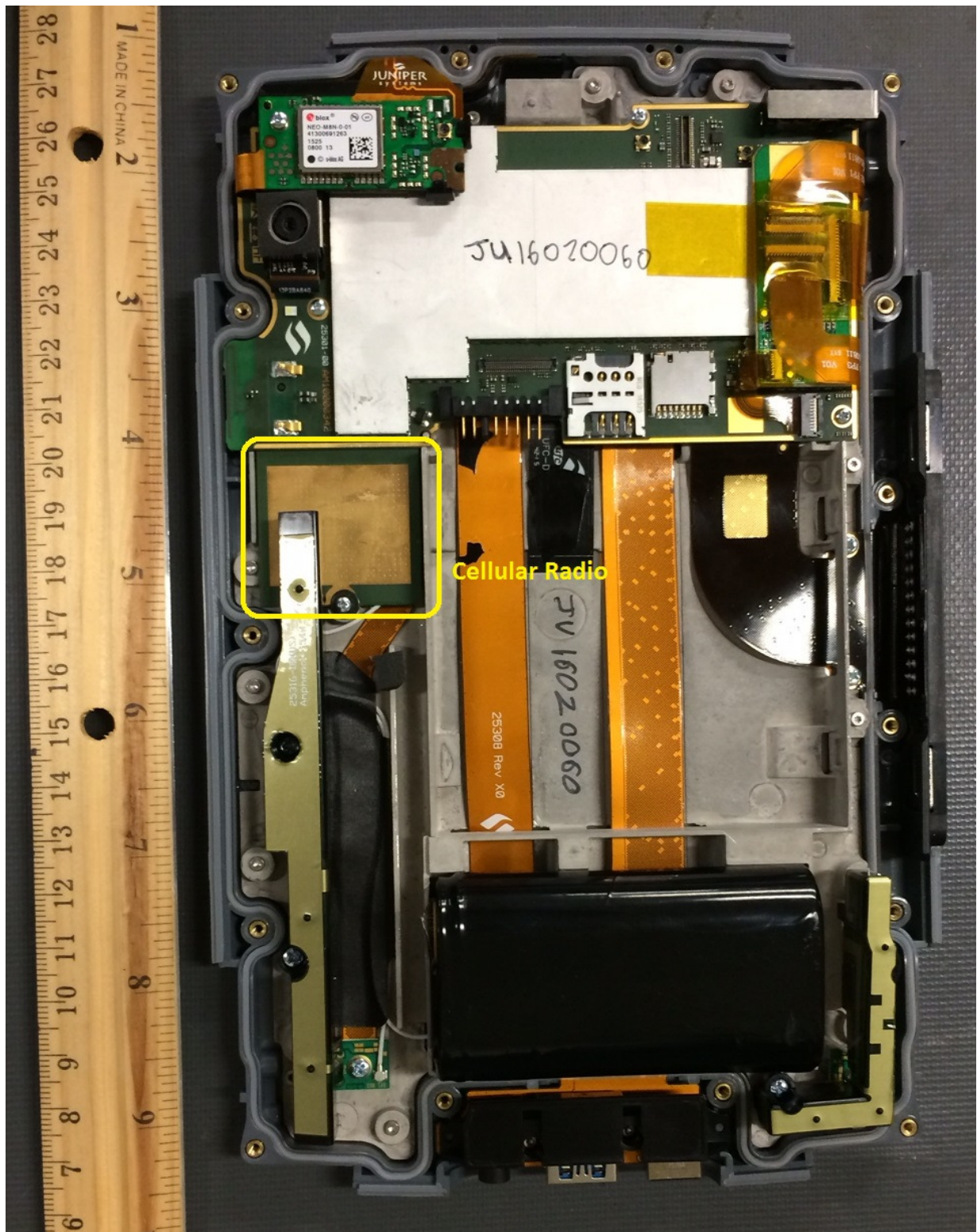
Figure 3: Assembled - View 1
