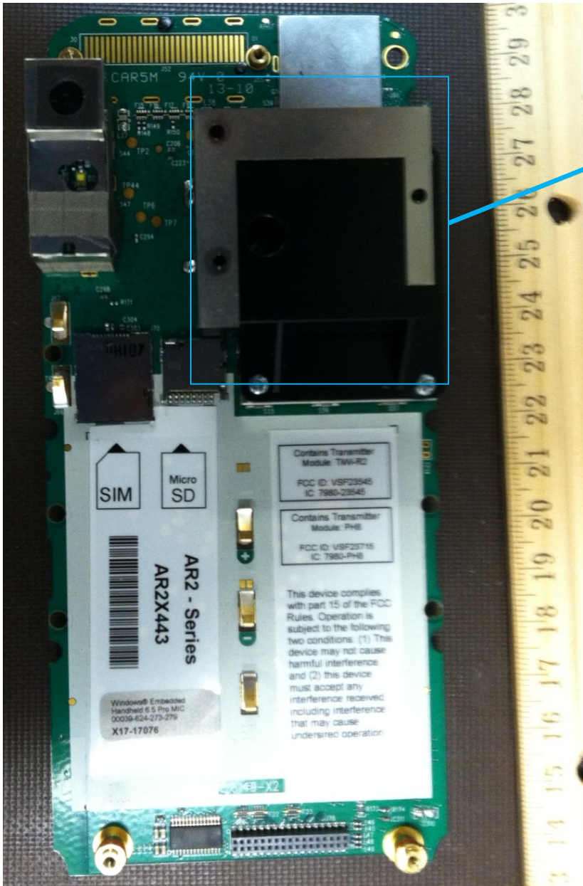
Antenna for PSV8 Radio Module (installed on top on the radio module mainboard)
