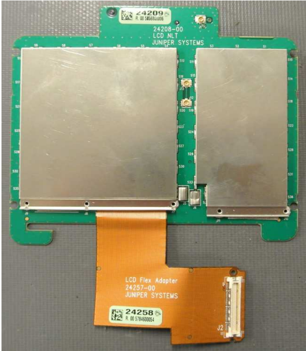
LCD adapter board (top) with shields and tail
