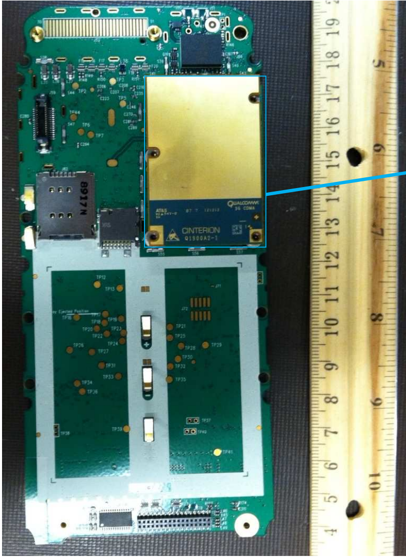
PH8-P Radio Module installed on mainboard
