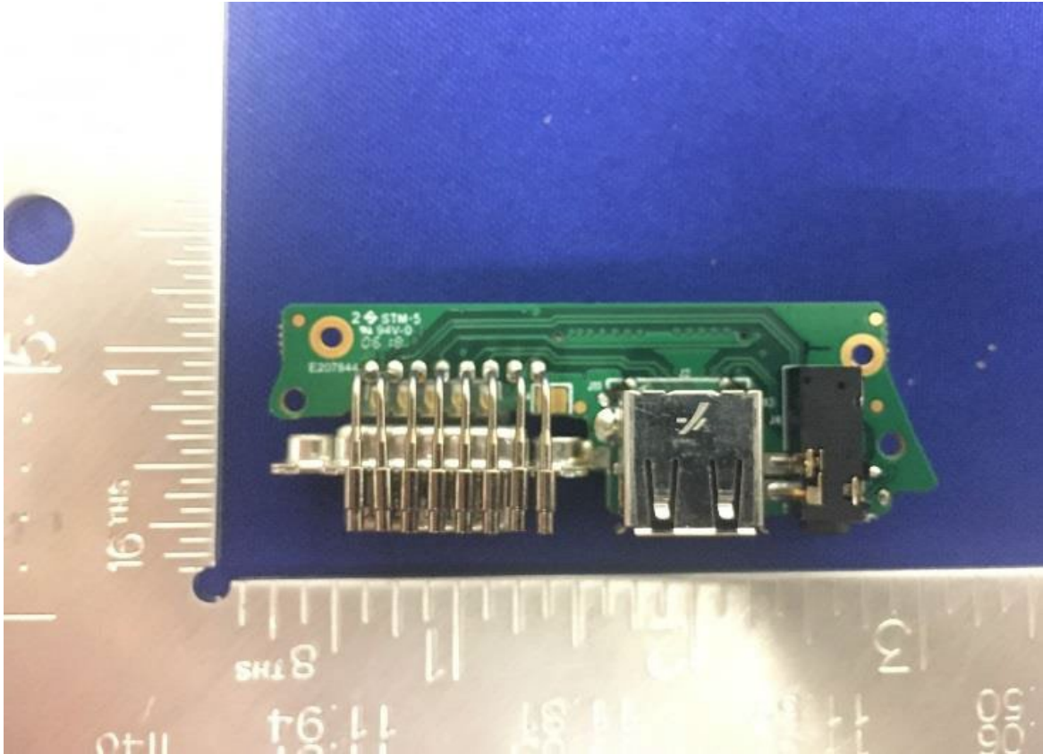
IO board - Back
