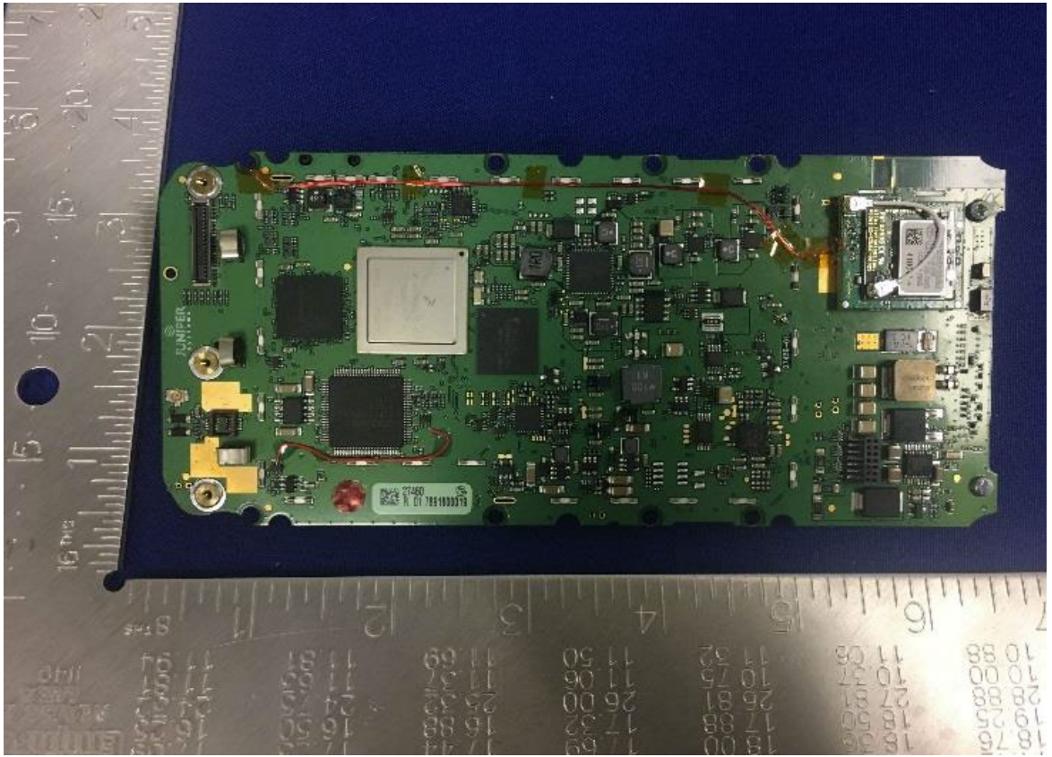
Main Board - Shields Removed
