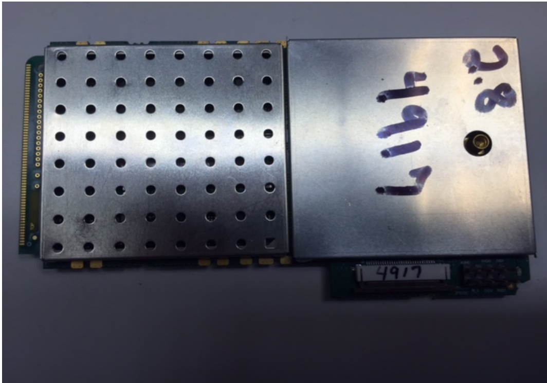
Panther Radio - Top with shields installed
