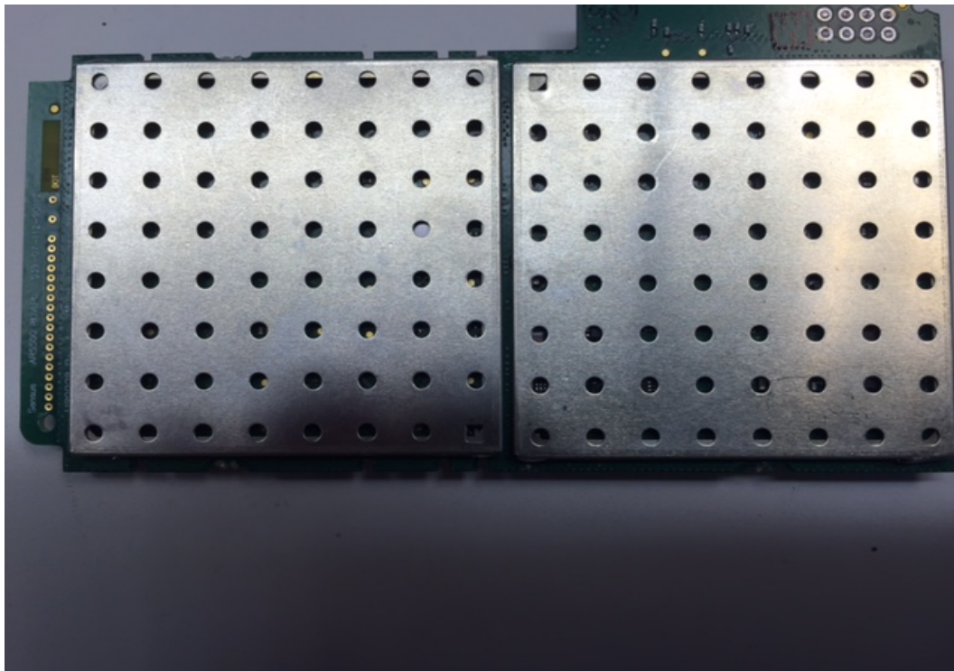
Panther Radio - Bottom with shields installed
