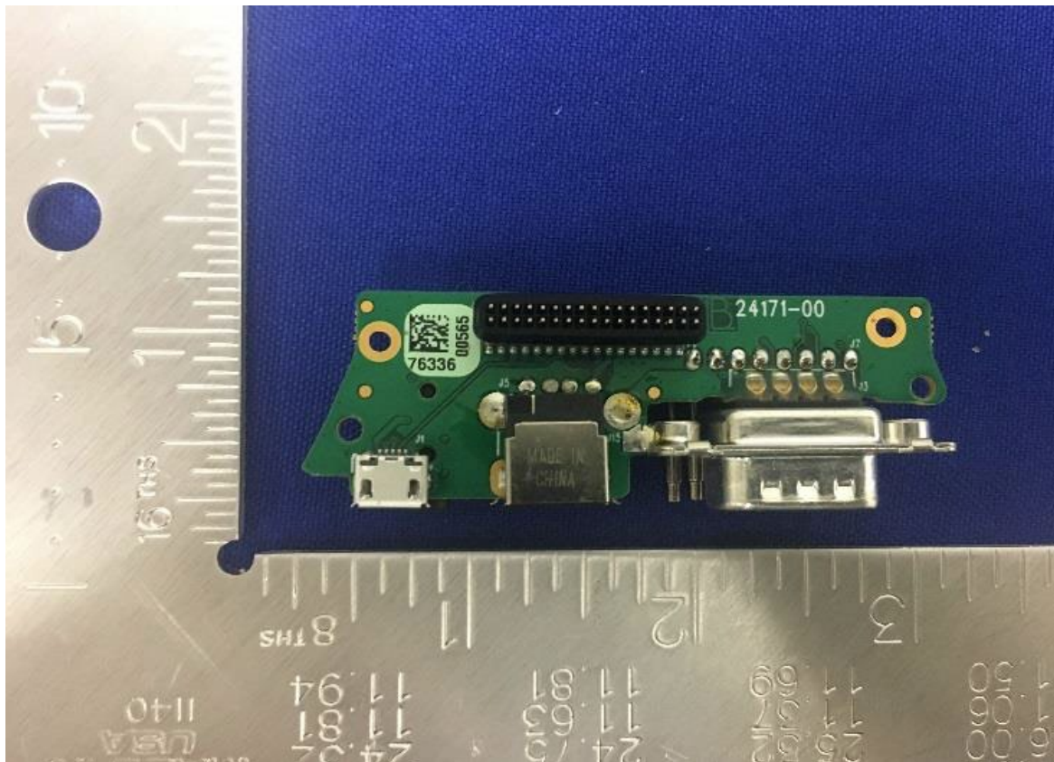
IO board - Front
