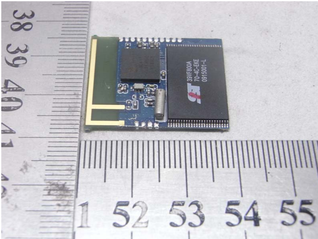
Internal of Bluetooth module-1
