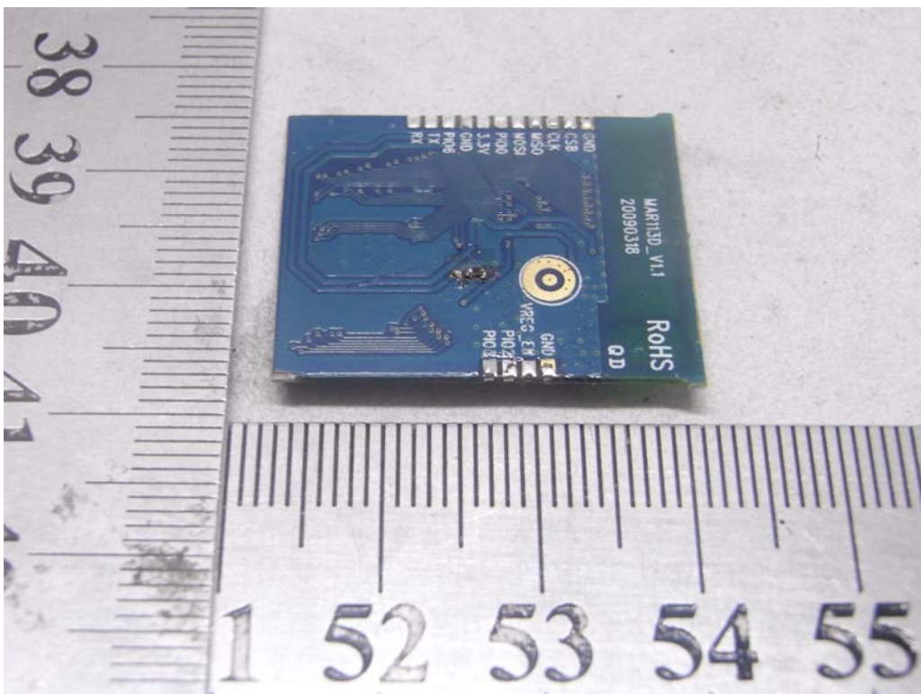
Internal of Bluetooth module-2
