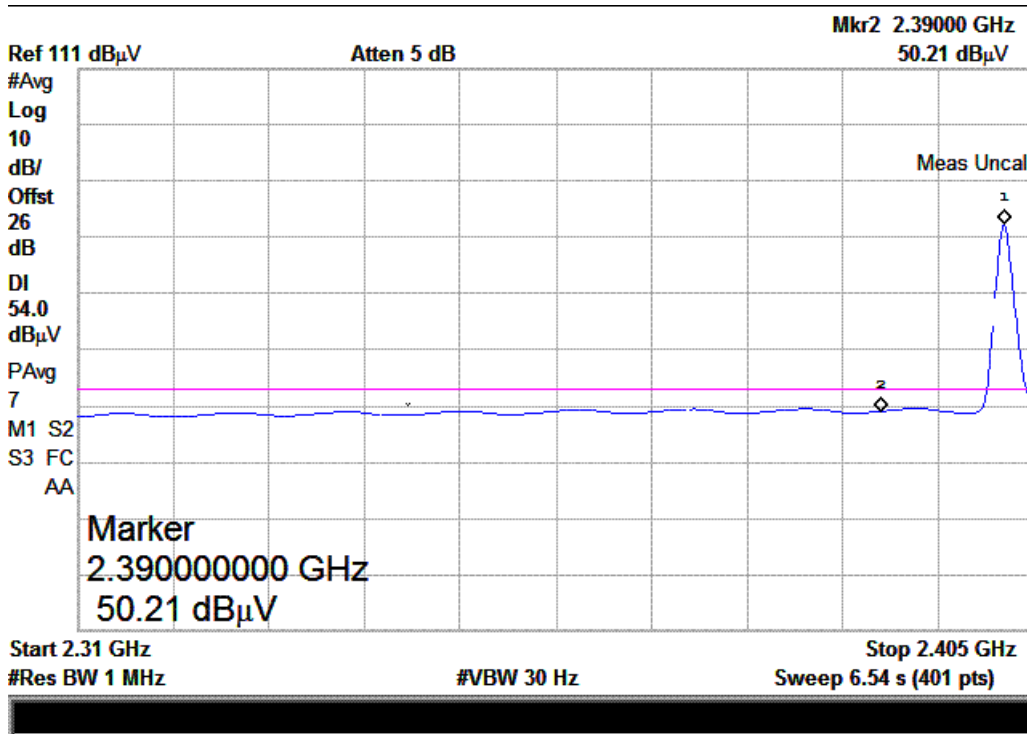
(Plot 15: Channel = 0, Detector Mode: Average, Polarity: Horizontal)
