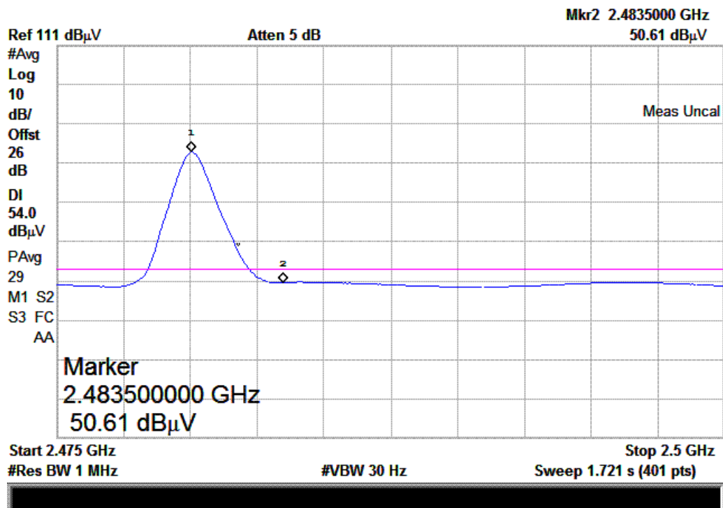
(Plot 18: Channel = 78, Detector Mode: Average, Polarity: Vertical)
