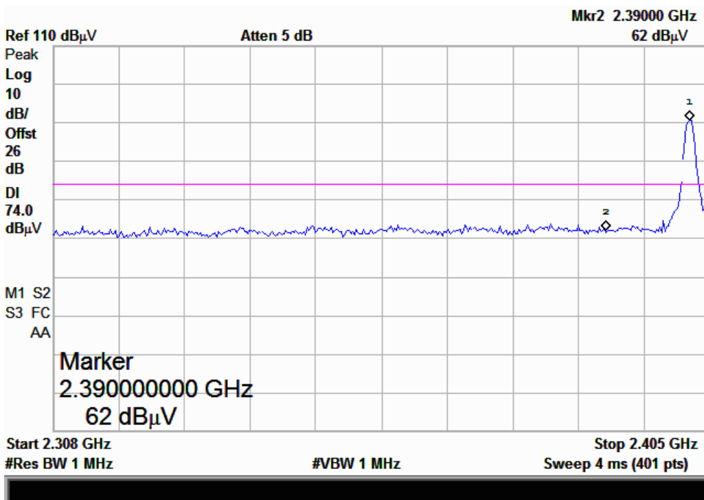
(Plot 11: Channel = 0, Detector Mode: Peak, Polarity: Horizontal)
