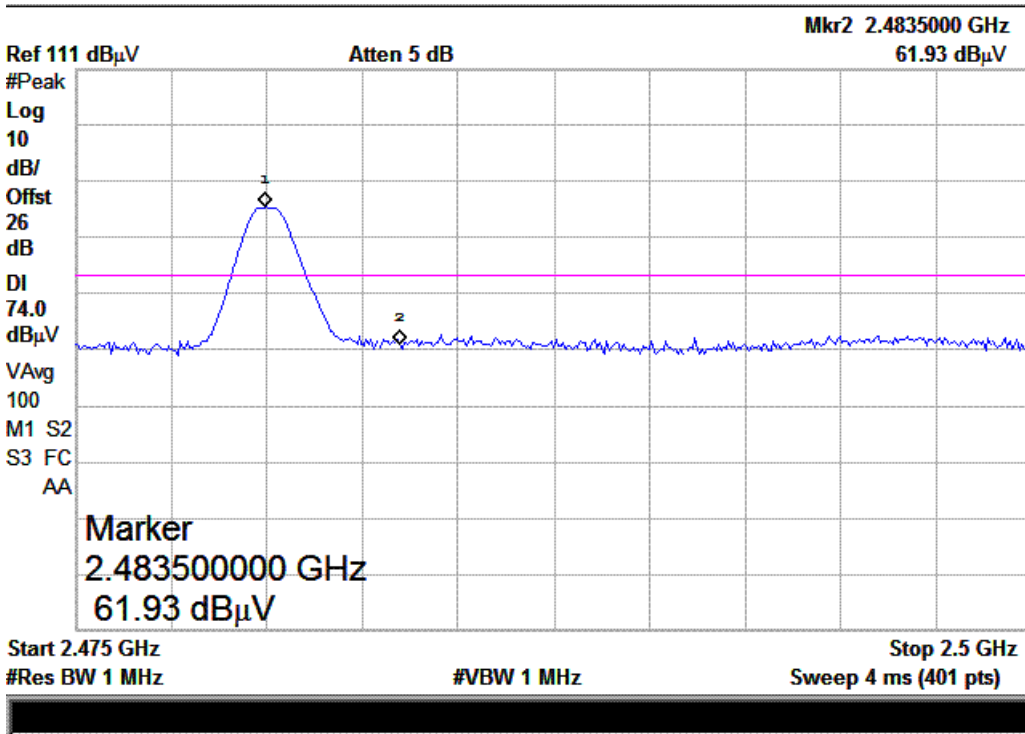
(Plot 13: Channel = 78, Detector Mode: Peak, Polarity: Horizontal)
