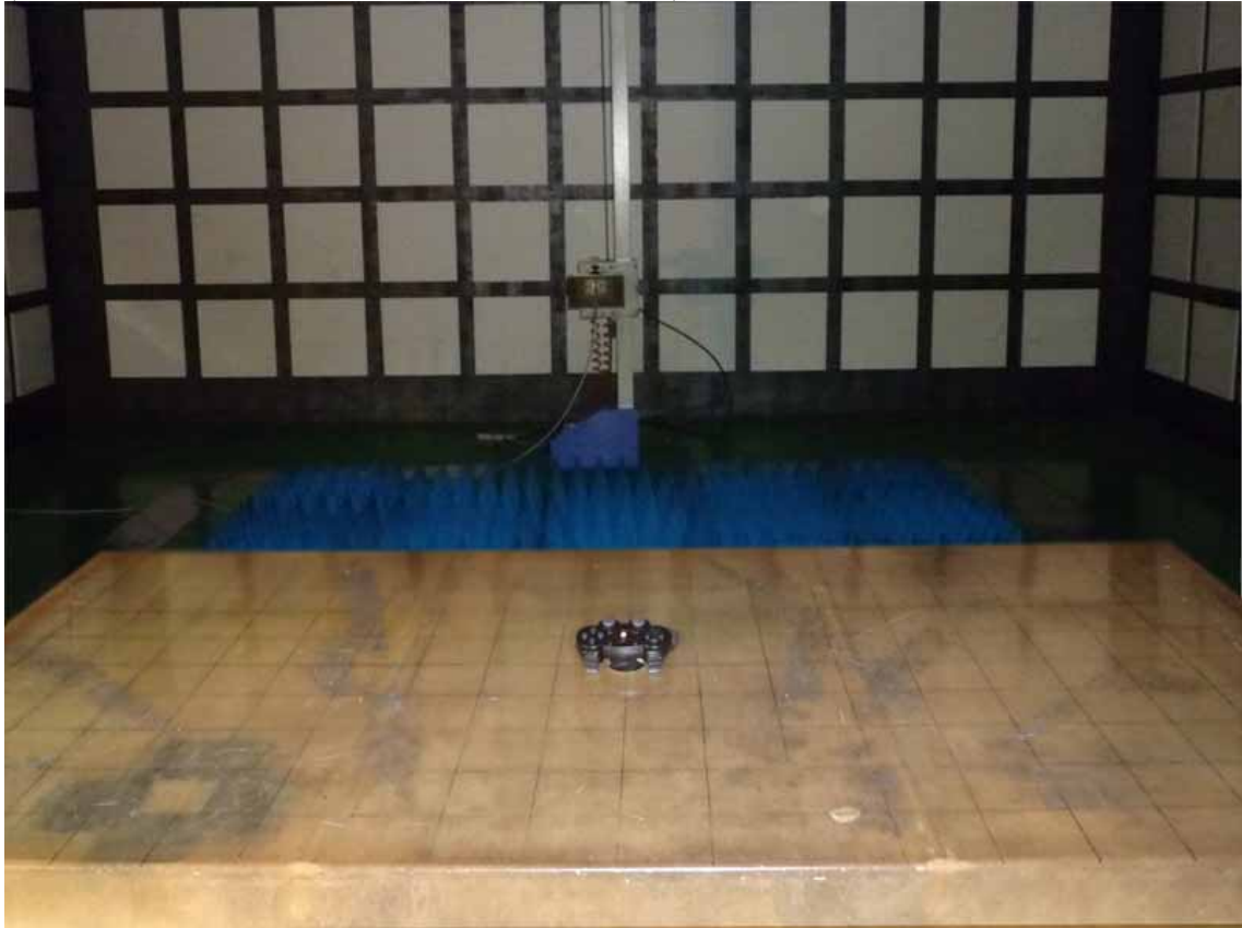
(At Anechoic 3m Chamber Test 1GHz –18GHz)
