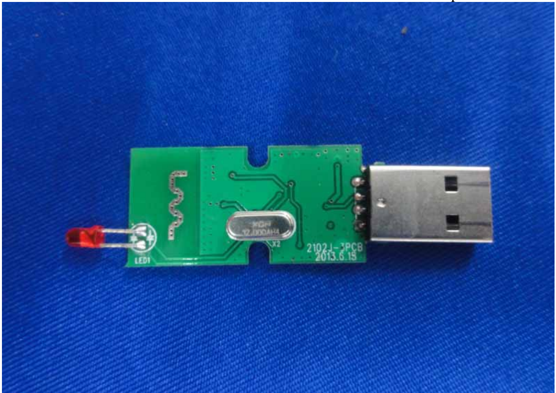
Figure 6 Component Side of the PCB
