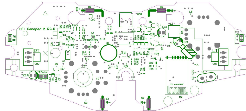
Top Silkscreen
