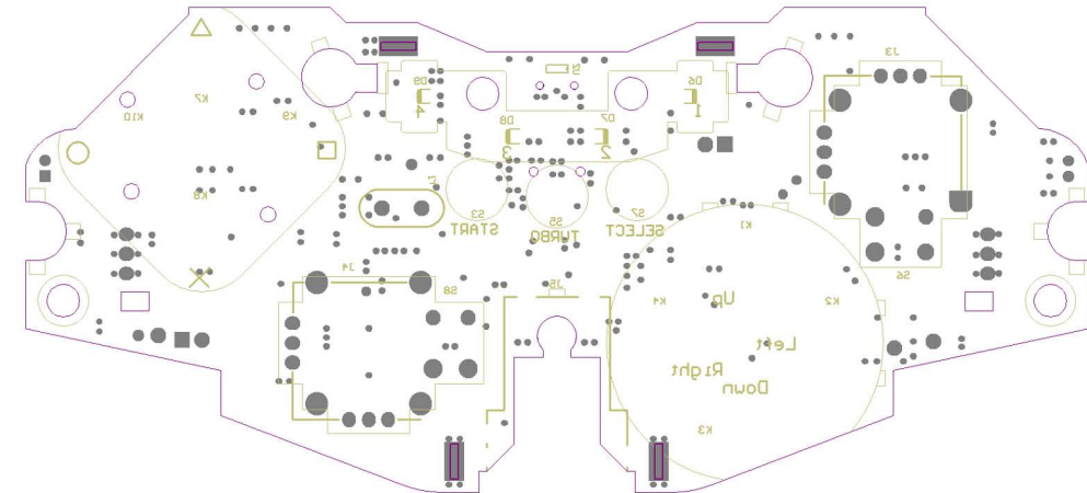
Bottom Silkscreen
