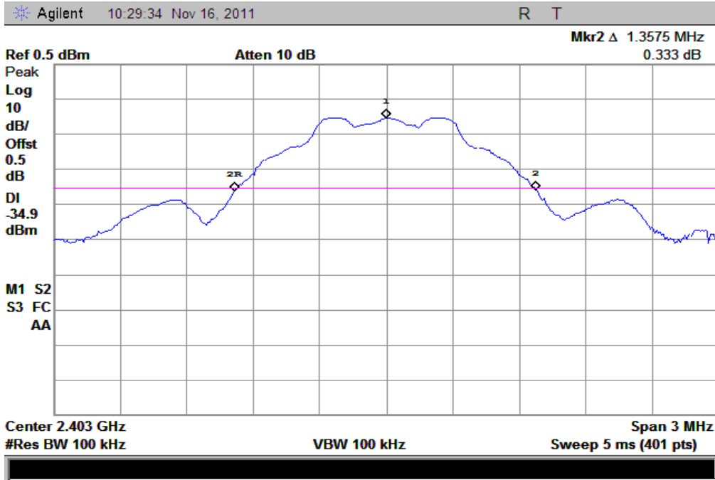
(Plot A: Channel = 2403 @ GFSK)
