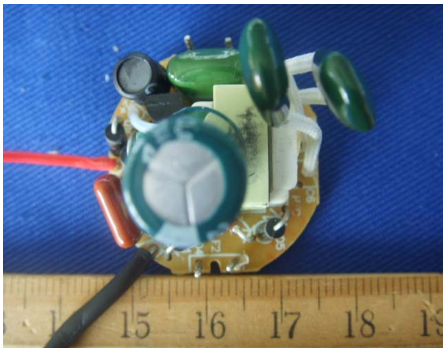
EUT –Components View (NHSZR13)
