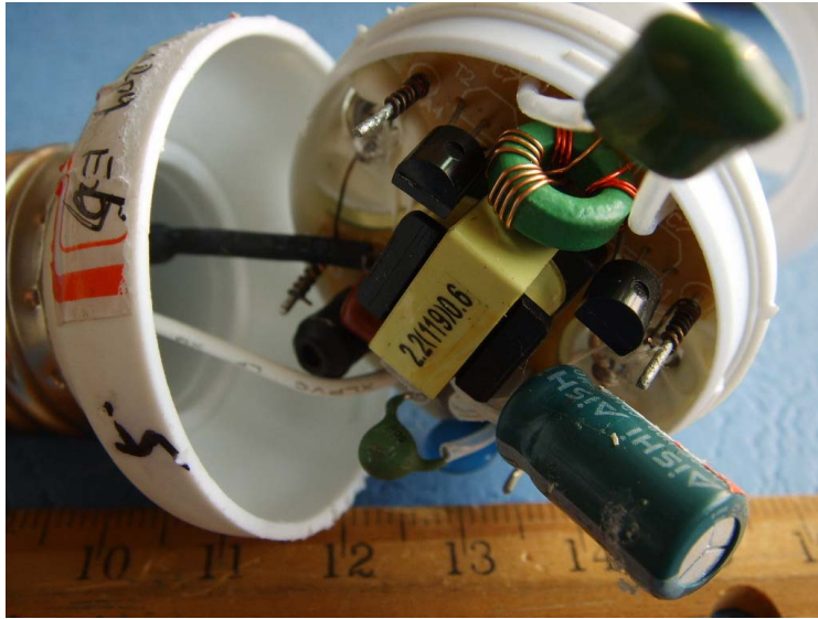
EUT – Uncovered View (NHSAR09)
