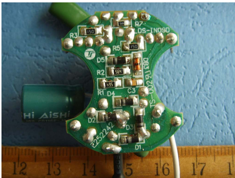
EUT–Solder View (NHSAR13)
