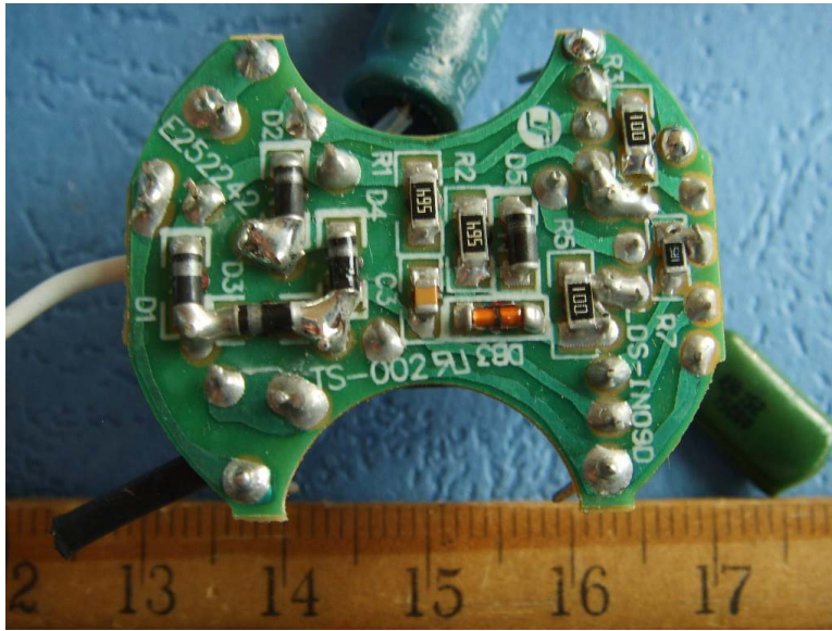
EUT-Solder View (NHSAR09)
