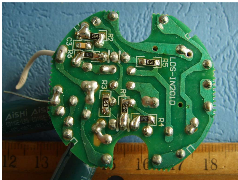
EUT–Solder View (NHSI20)
