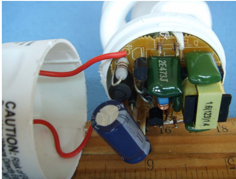
EUT – Uncovered View (NHSCT13)
