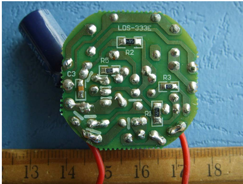
EUT-Solder View (NHSCT13)
