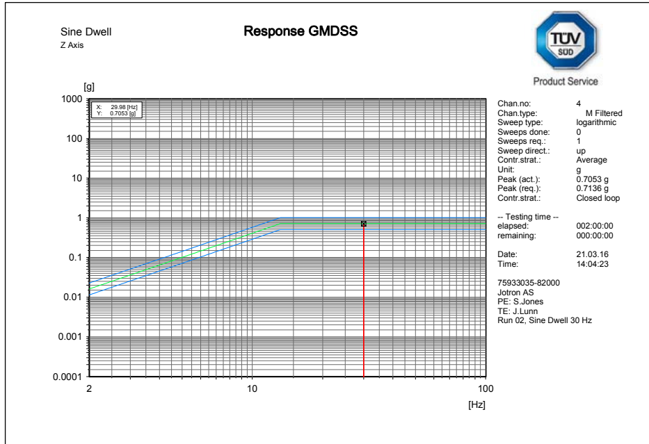
Z axis endurance run (control plot)
