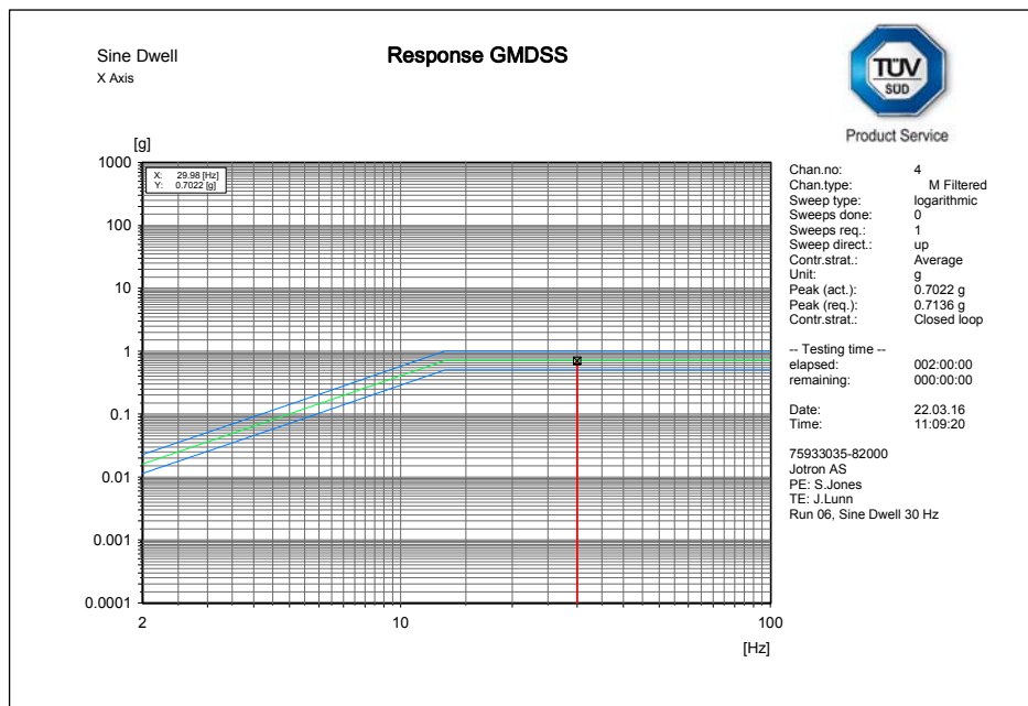
X axis endurance run (EUT plot)
