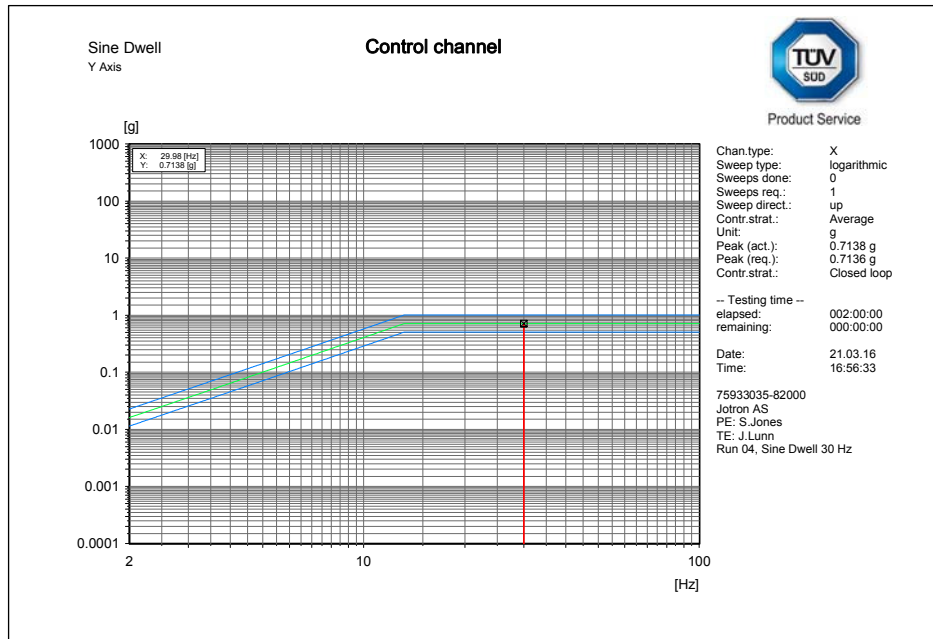
Y axis endurance run (control plot)
