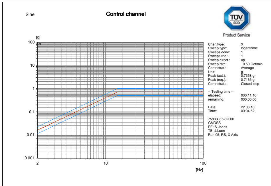
X axis resonance search (control plot)
