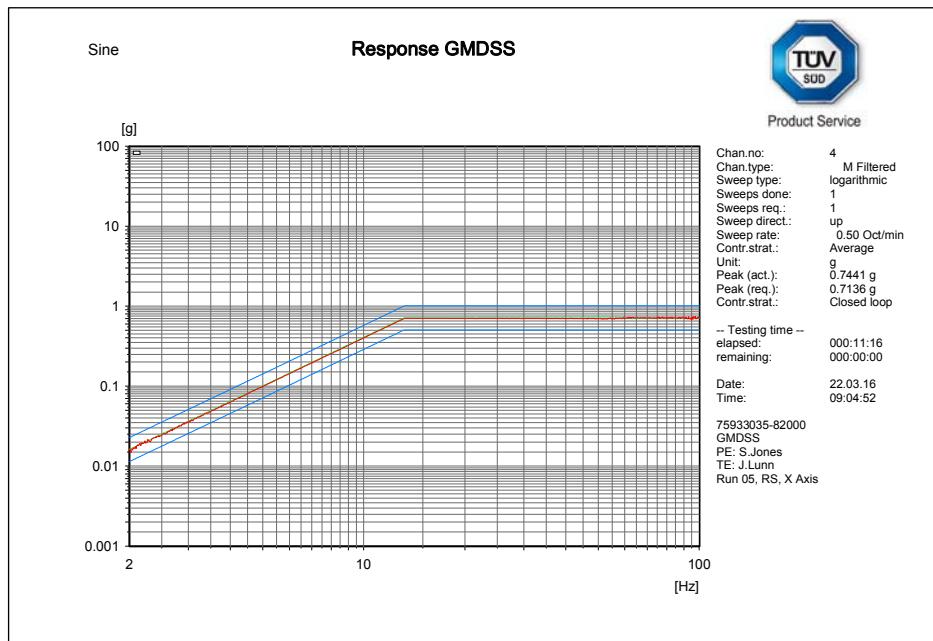
X axis resonance search (EUT plot)
