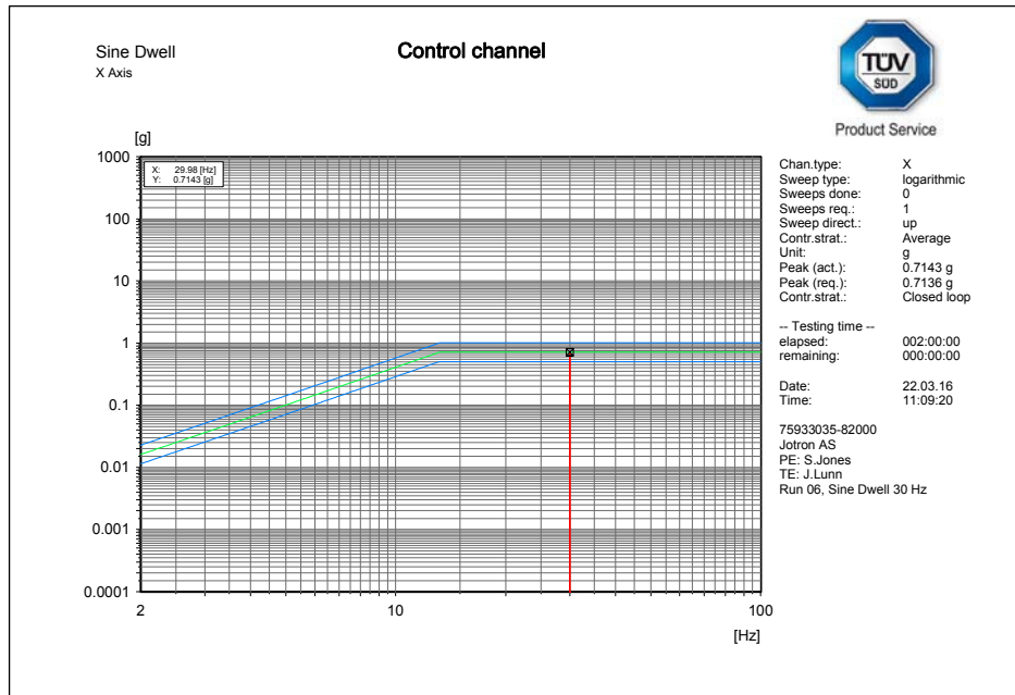
X axis endurance run (control plot)
