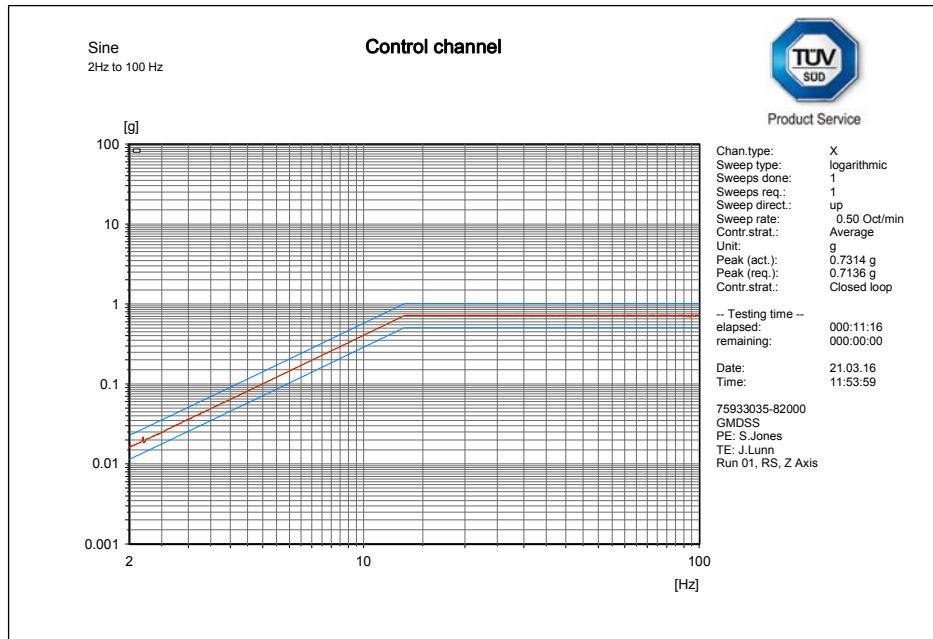
Z axis resonance search (control plot)
