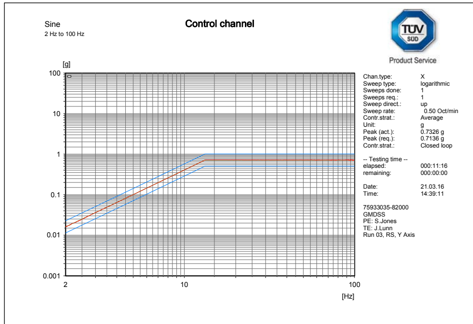
Y axis resonance search (control plot)
