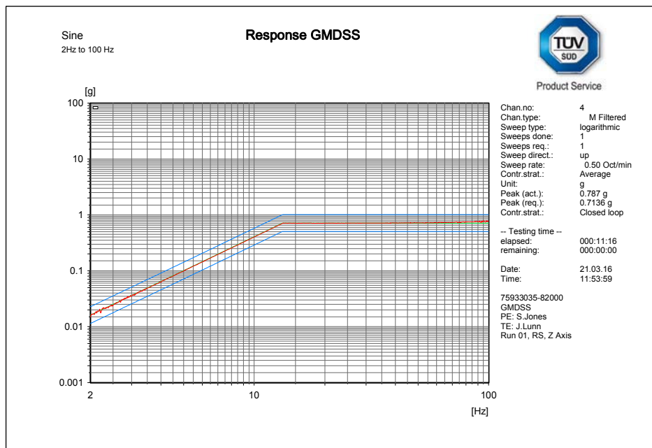
Z axis resonance search (EUT plot)
