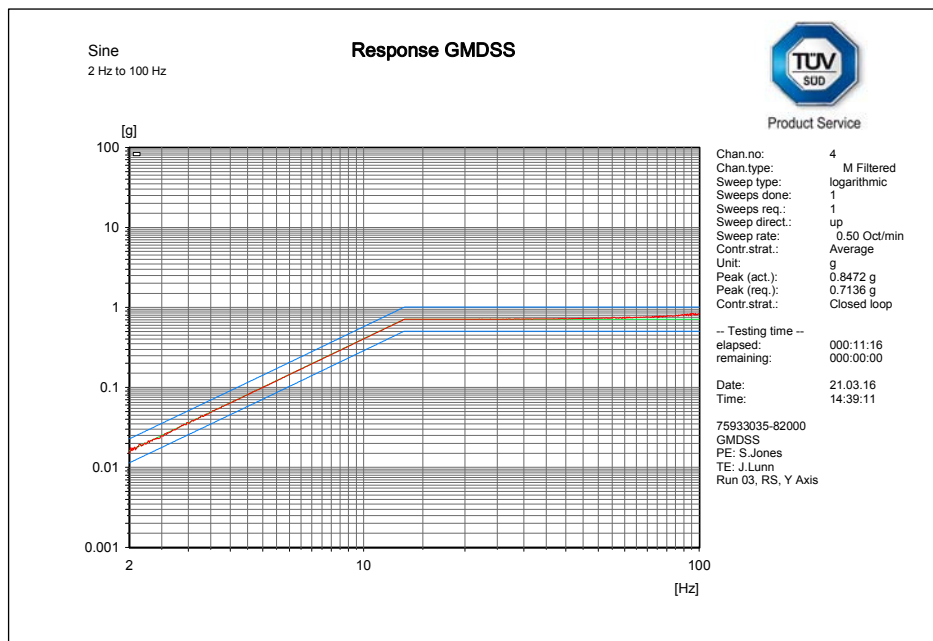
Y axis resonance search (EUT plot)
