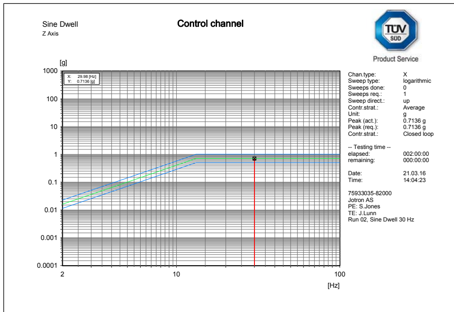
Z axis endurance run (EUT plot)
