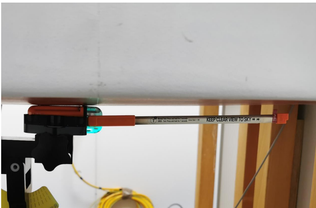
Figure 3. Back of the DUT facing phantom, 0mm
