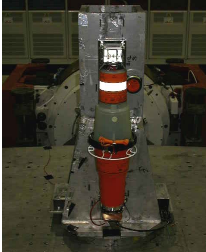
Test Set-up
