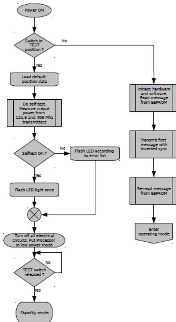
Figure 1: Self-Test flowchart
