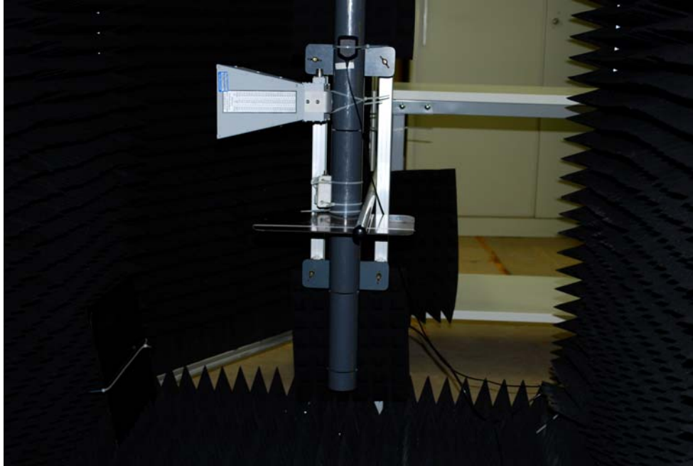
L-Band interference test – GPS antenna unit 3
