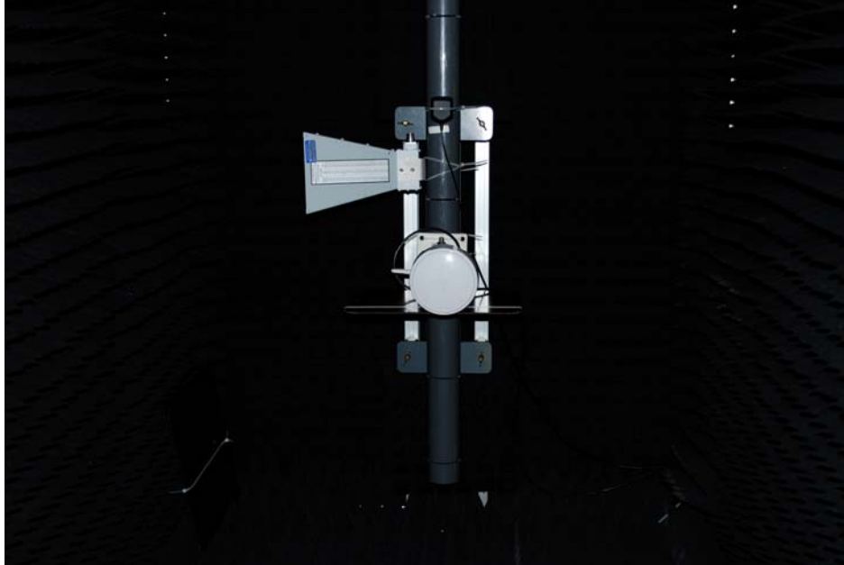
L-Band interference test – GPS antenna unit 1
