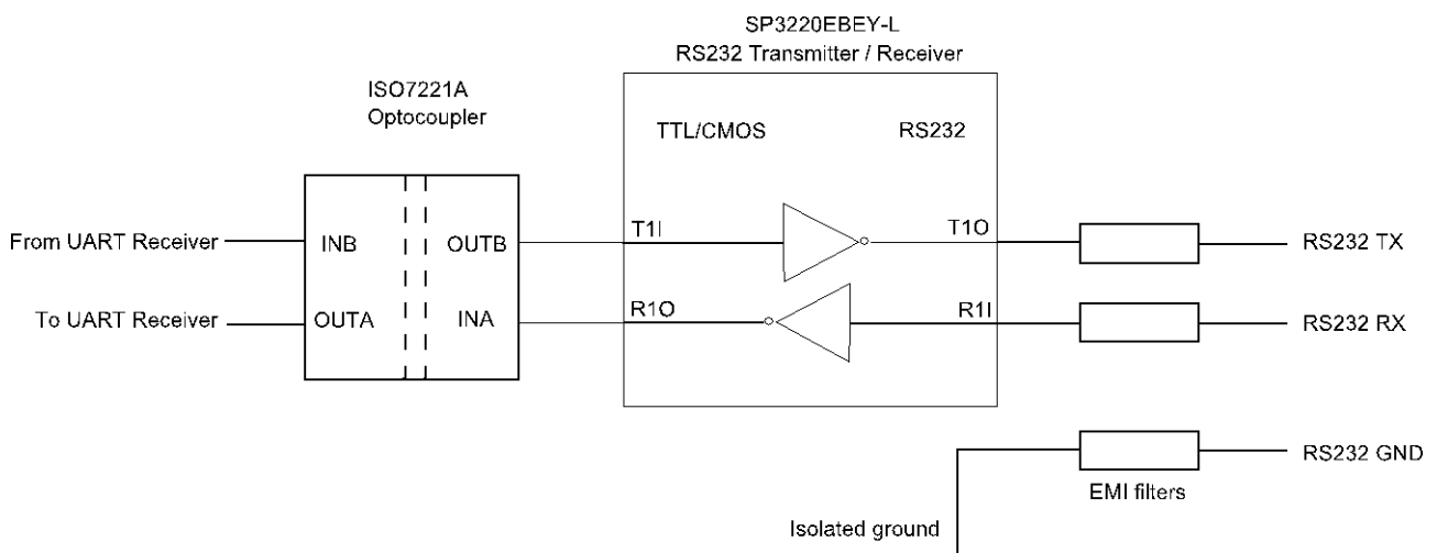
Figure 2: Simplified diagram of the RS232 interface
