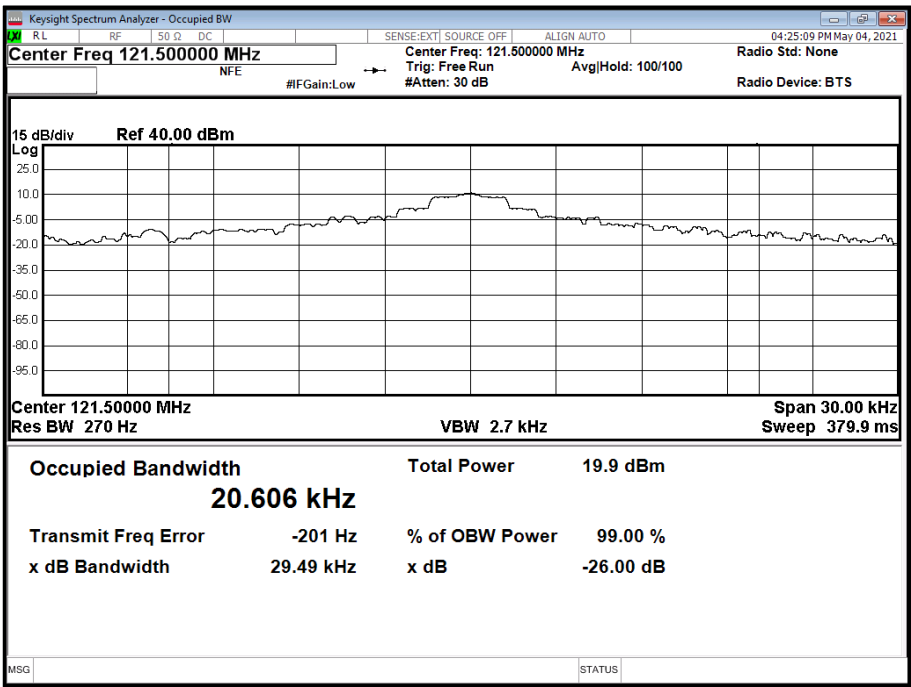
Figure 1 - Occupied Bandwidth
