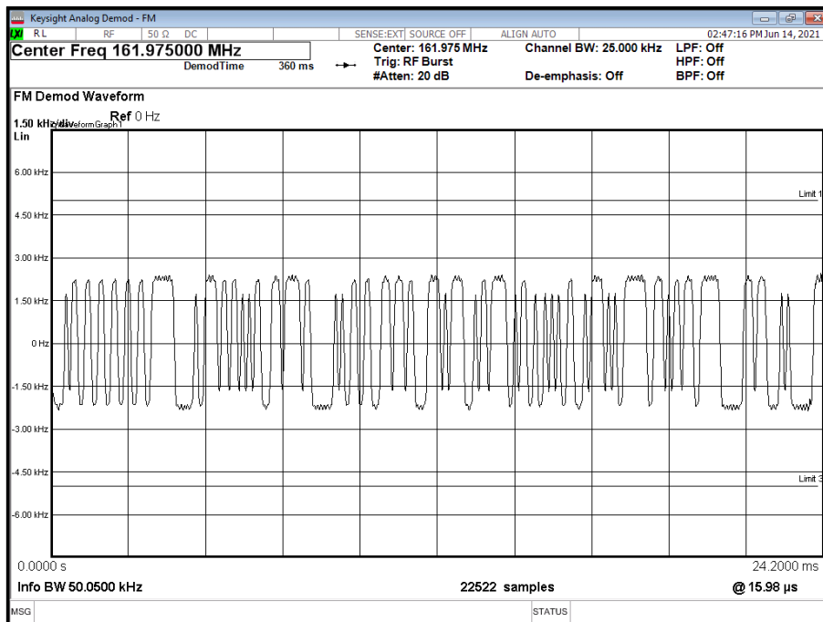
Figure 17- 161.975 MHz - PRBS
