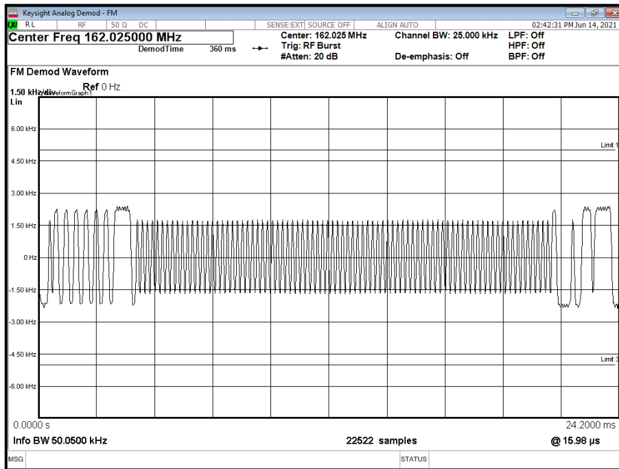
Figure 18 - 162.025 MHz - 01010101
