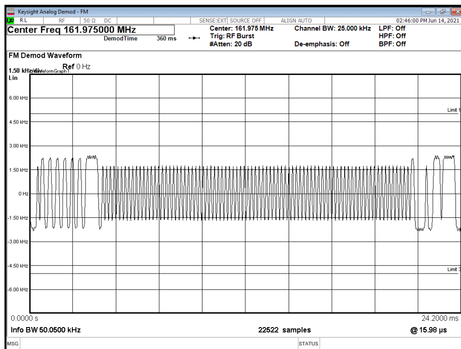
Figure 15 - 161.975 MHz - 01010101
