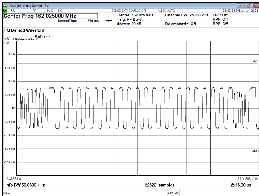
Figure 19- 162.025 MHz - 00001111
