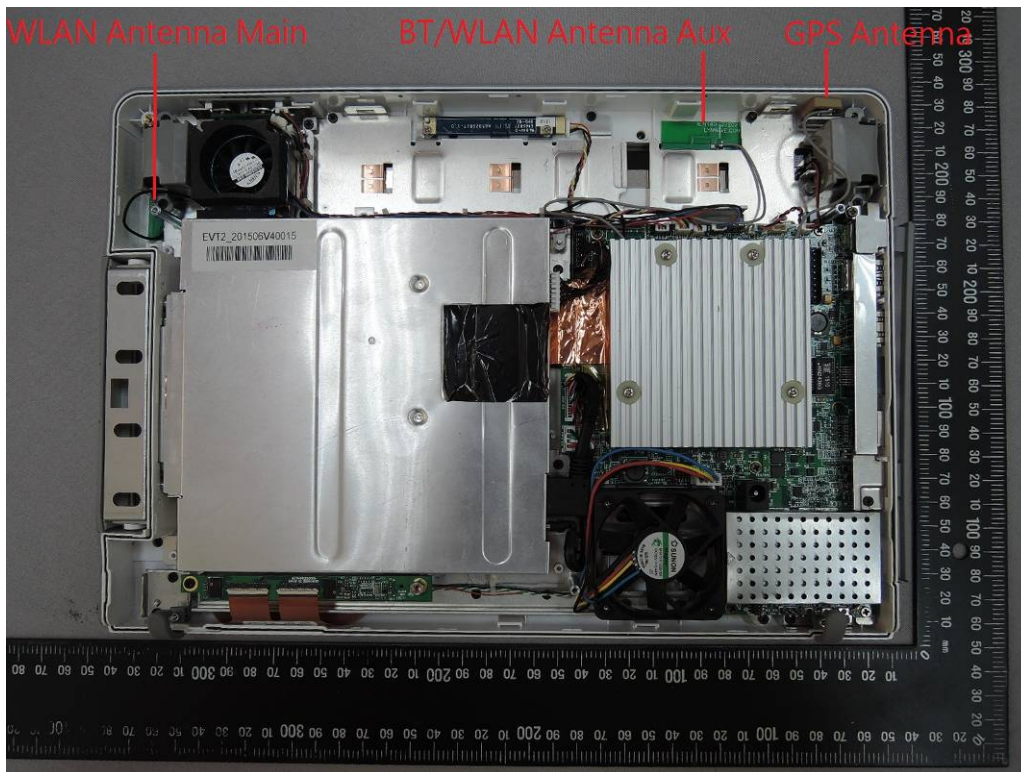
BT/WLAN/GPS Antenna
