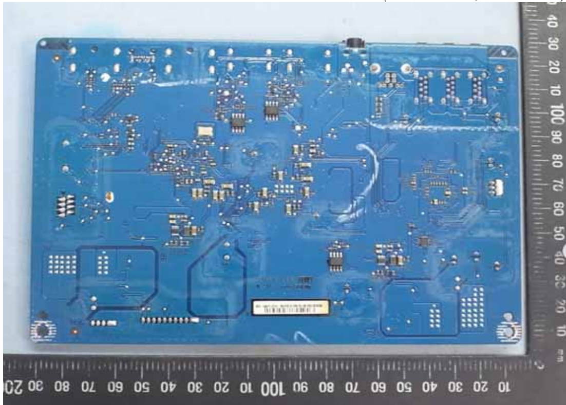
Figure 14 Internal View (Main Board, Back View)
