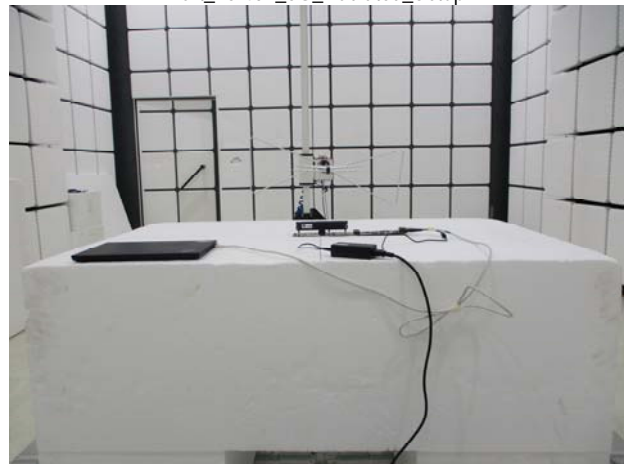
Part_15.407_5G_Radiated_Setup
