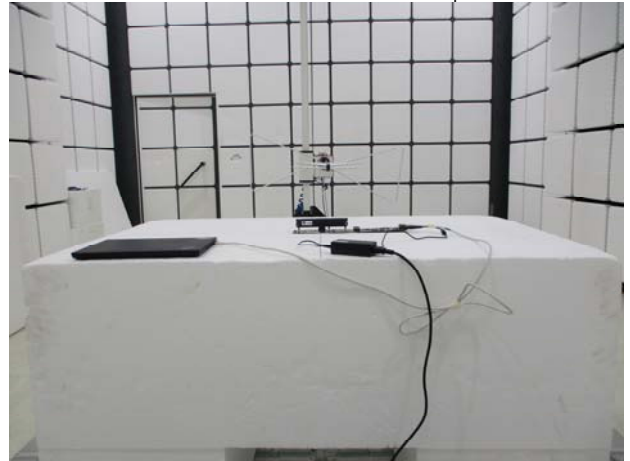
Part_15.247_BT_Radiated_Setup
