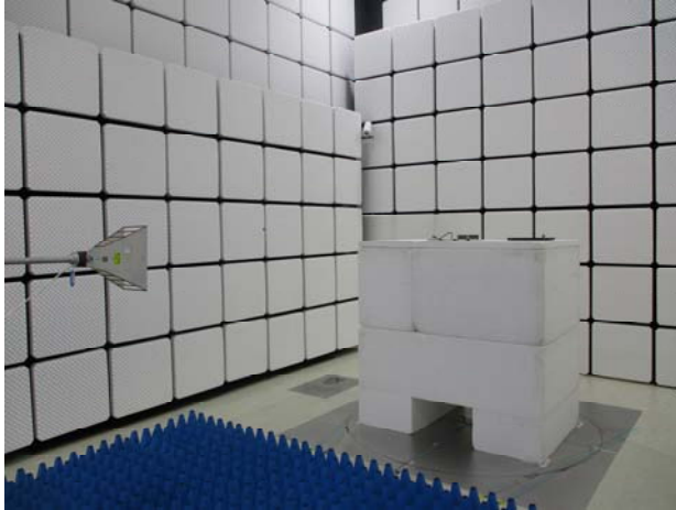
RSS-247 (5G_Band 1 and 2)_Radiated_Setup
