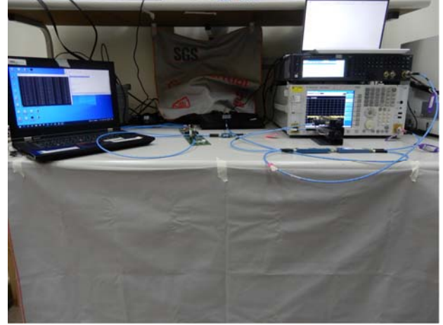
Part_15.407_5G_Normal_DFS_Setup
