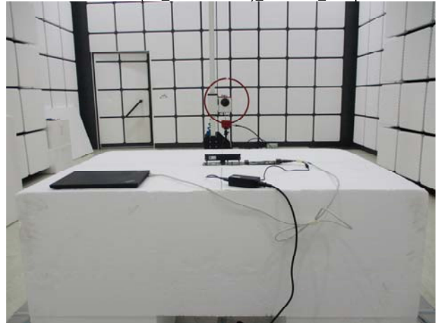
RSS-247 (5G_Band 1 and 2)_Radiated_Setup
