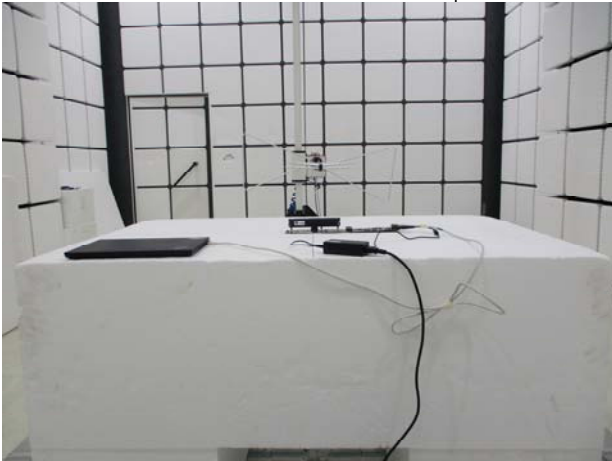
Part_15.247_2.4G_Radiated_Setup
