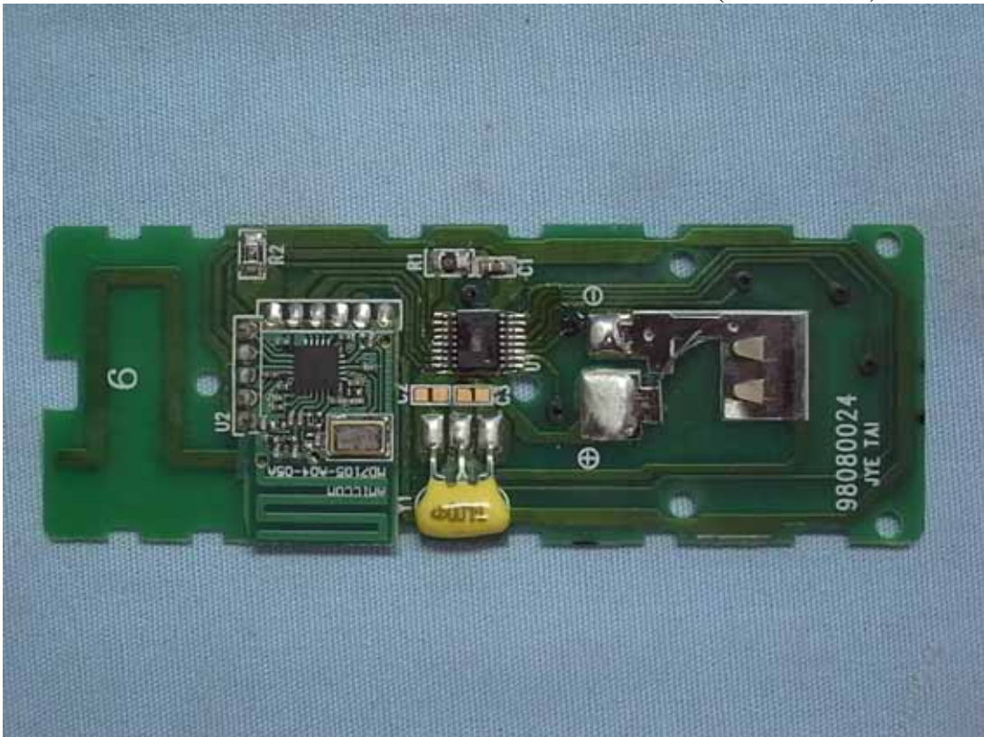
Figure 4 Internal View (PCB Board, Front View)
