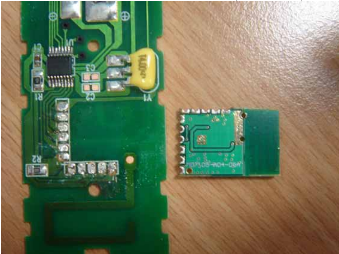
Figure 6 Internal View (Module Board, Back View)
