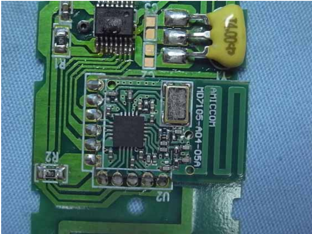
Figure 5 Internal View (Module Board, Front View)
