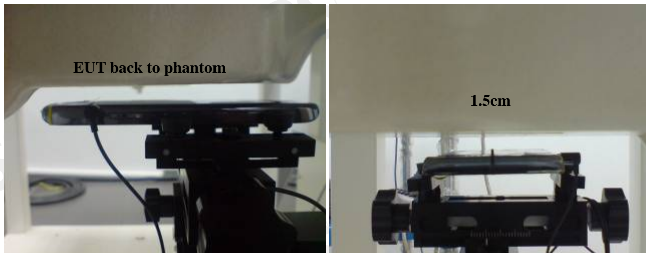
Fig.9 Body worn- EUT back to flat phantom and distance between flat phantom and mobile phone is 1.5 cm with headset
