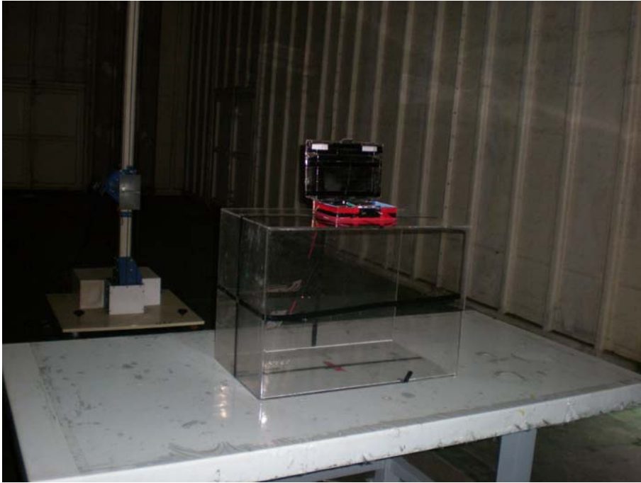
Back View of Radiated Test (Horn) (Zoom Out)
