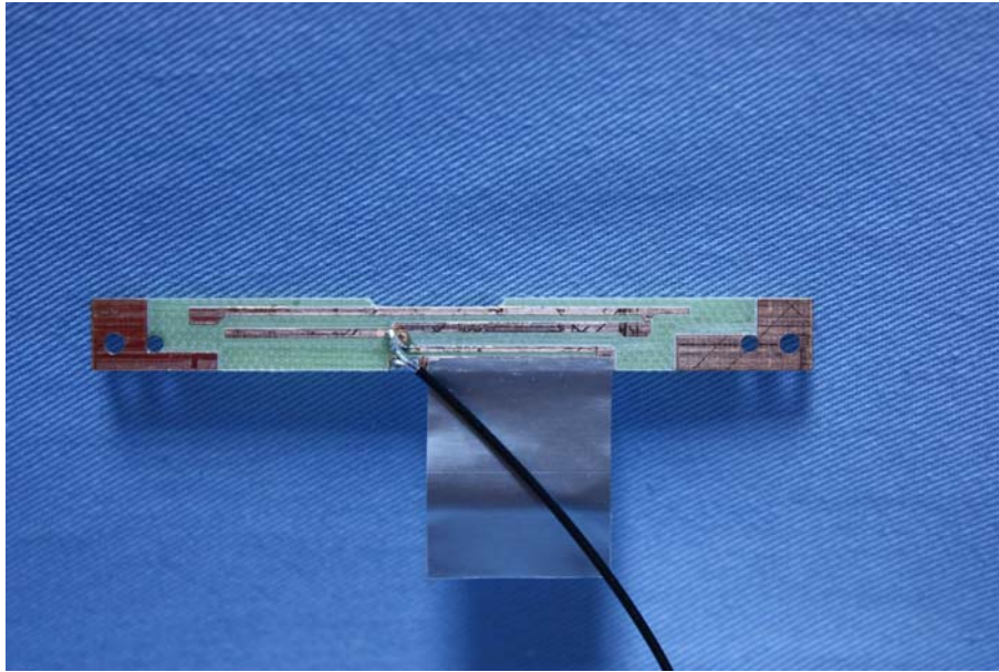
(17) EUT Photo(M/N:M760S)
