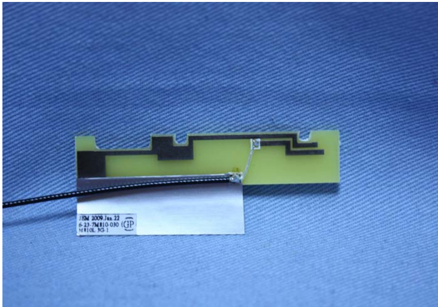
(23) EUT Photo(M/N:M810L-1-2) -MFR:Joinsoon
