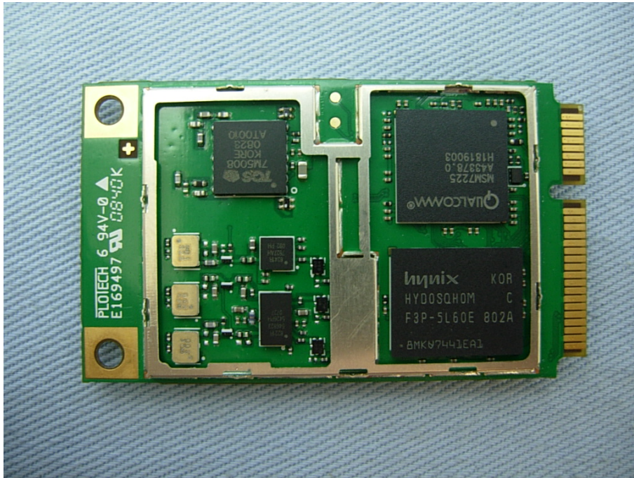
(10) EUT Photo(M/N:M740S)-Main Antenna
