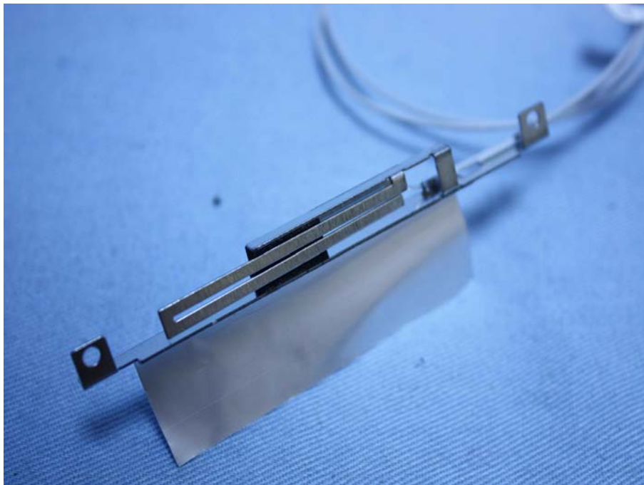
(26) EUT Photo(M/N:TN120R/T)
