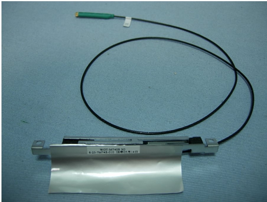
(19) EUT Photo(M/N:M740J)
