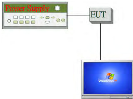
Fig. 2-1 Conducted Emission Configuration
