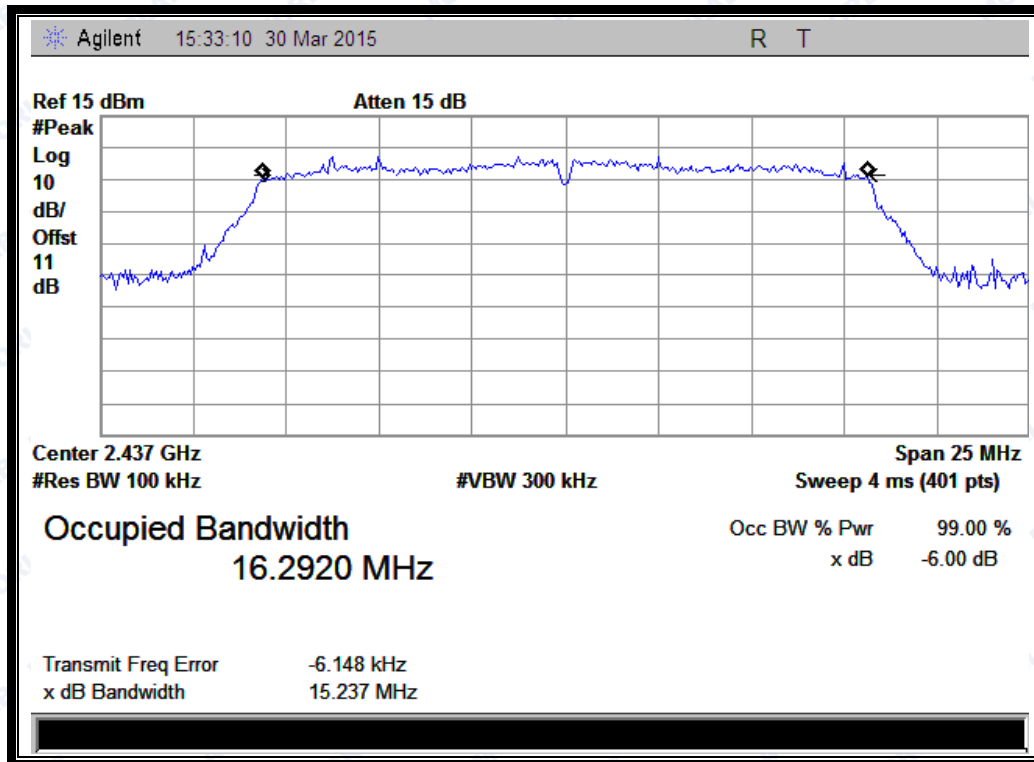
(Channel 6: 2437MHz @ 802.11g)
