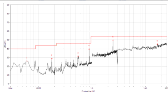
(Antenna Horizontal, 30MHz to 25GHz)
