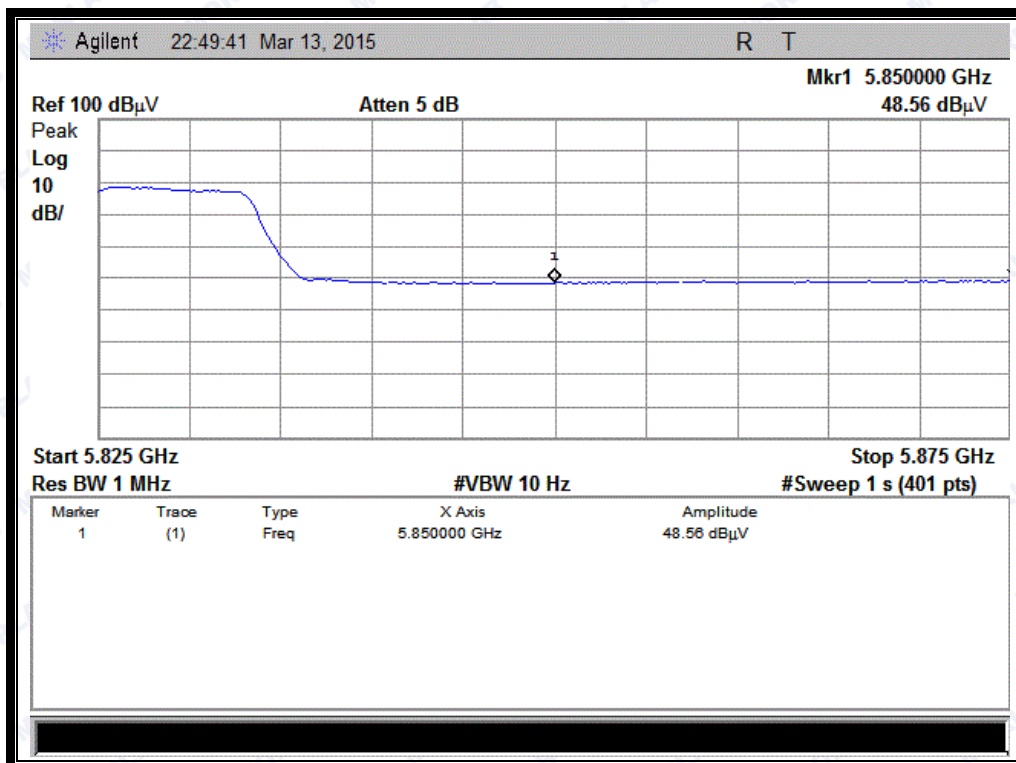
(Channel = 165 AVG @ 802.11a)
