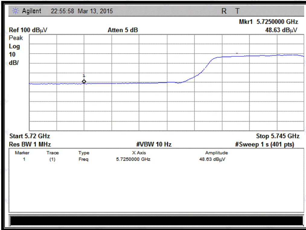
(Channel = 149 AVG @ 802.11n-20MHz)
