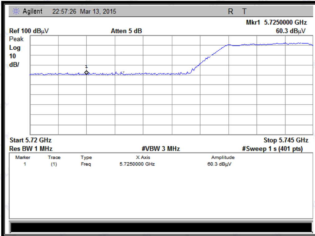
(Channel = 149 PEAK @ 802.11a)
