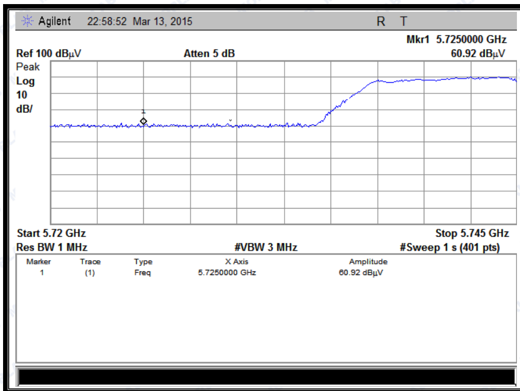
(Channel = 149 PEAK @ 802.11n-20MHz)
