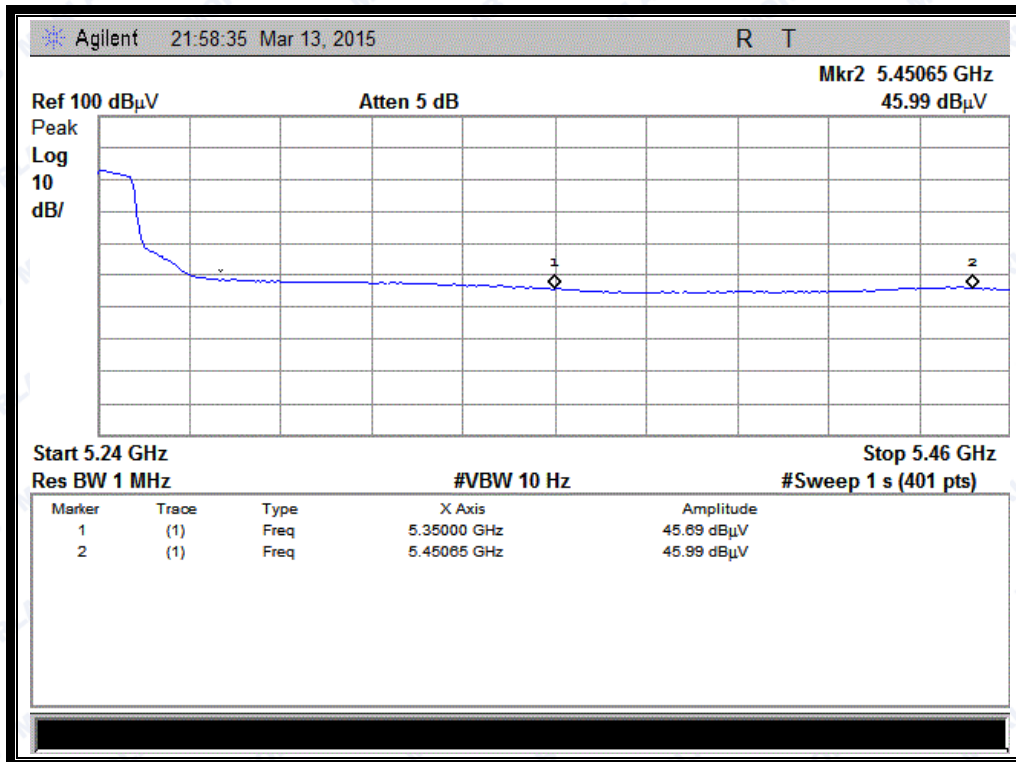
(Channel = 48 AVG @ 802.11a)
