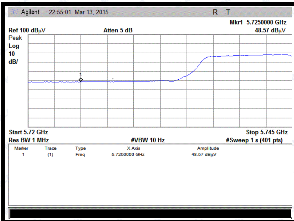
(Channel = 149 AVG @ 802.11a)
