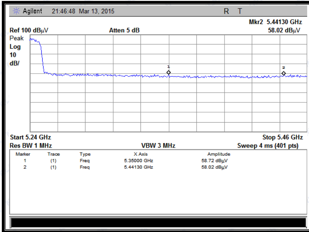
(Channel = 48 PEAK @ 802.11a)
