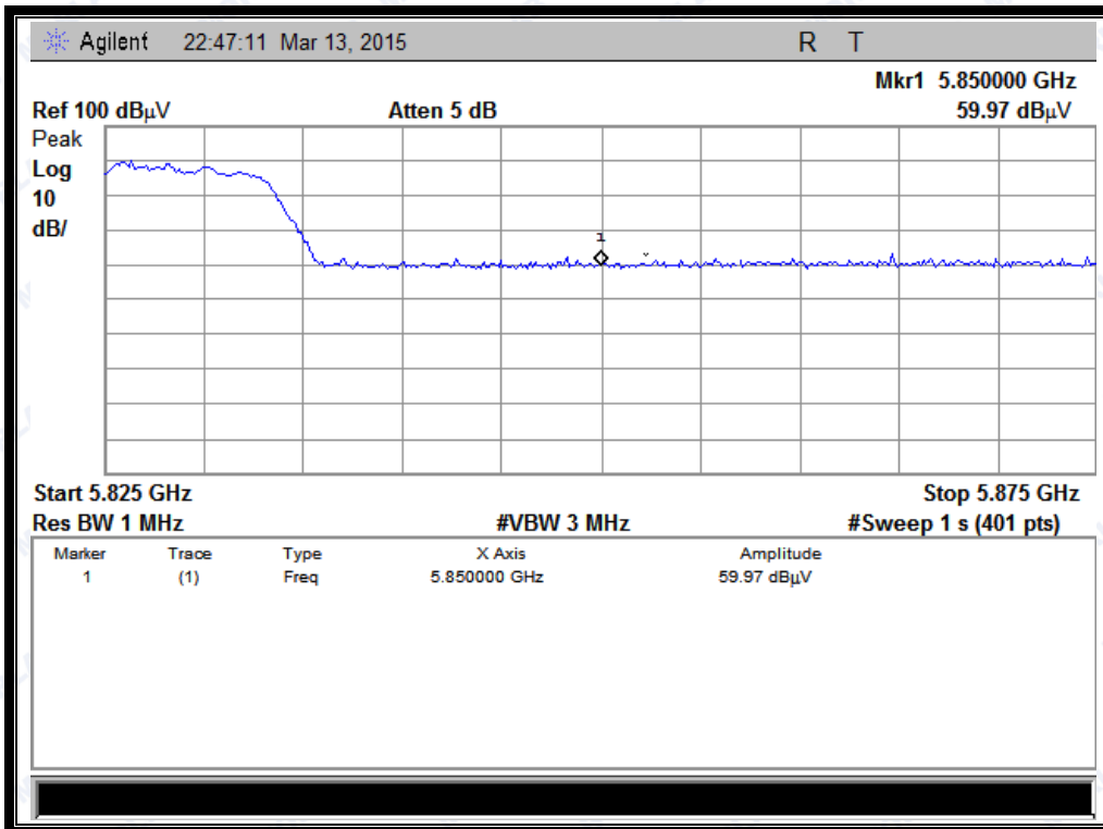
(Channel = 165 PEAK @ 802.11n-20MHz)
