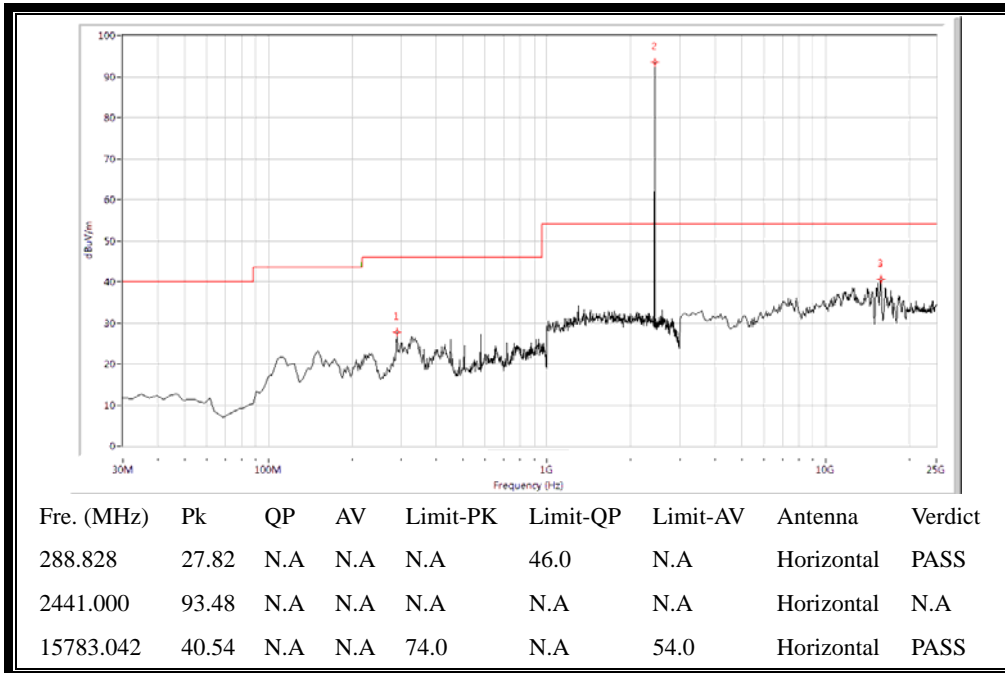
(30MHz to 25GHz, Antenna Horizontal @ GFSK, channel 39)
