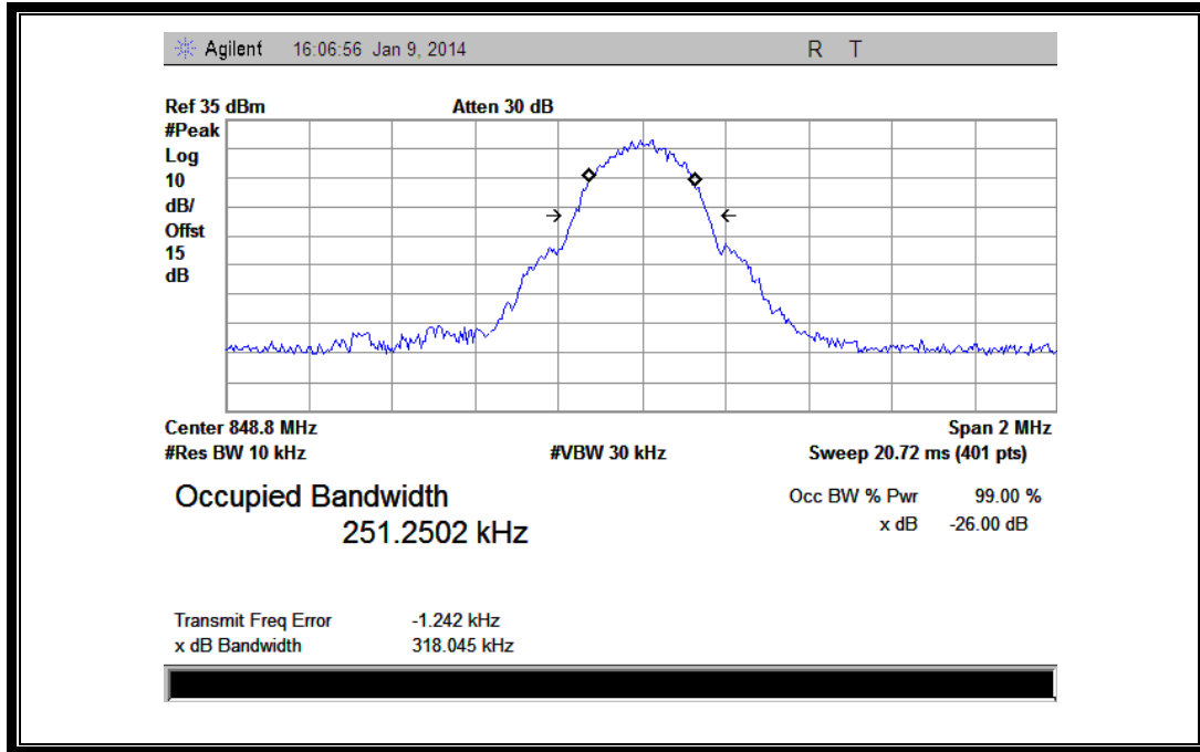
(Plot A1:GSM 850MHz Channel = 251)
