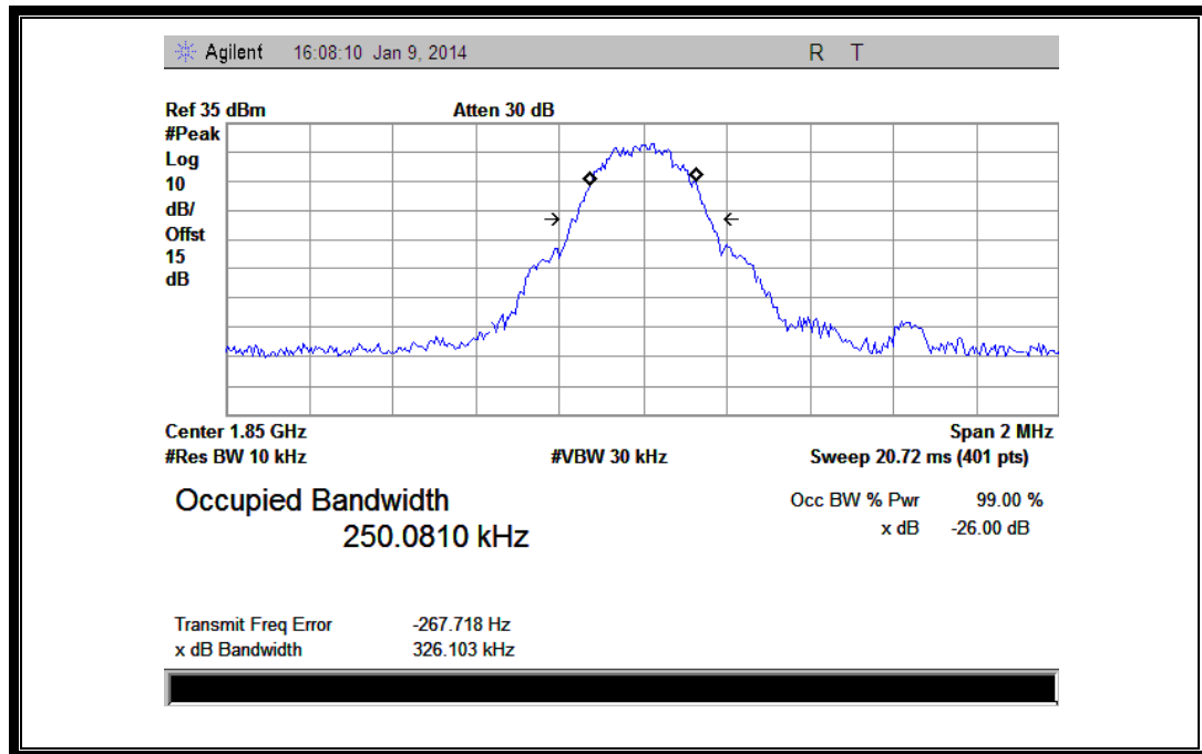
(Plot B1: GSM 1900MHz Channel = 512)
