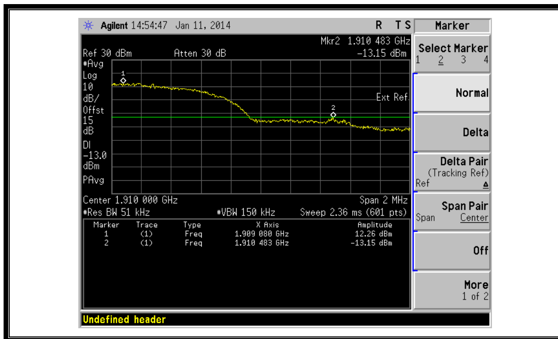
(Plot T: HSPA+ 1900 Channel = 9538)
