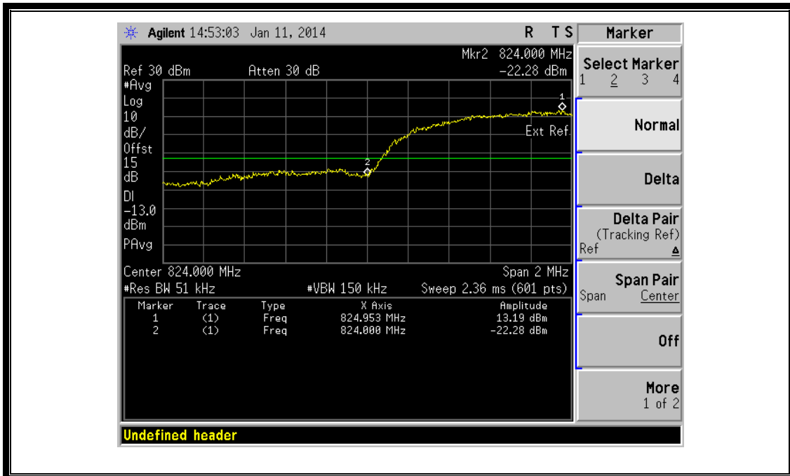
(Plot Q: HSPA+ 850 Channel = 4132)
