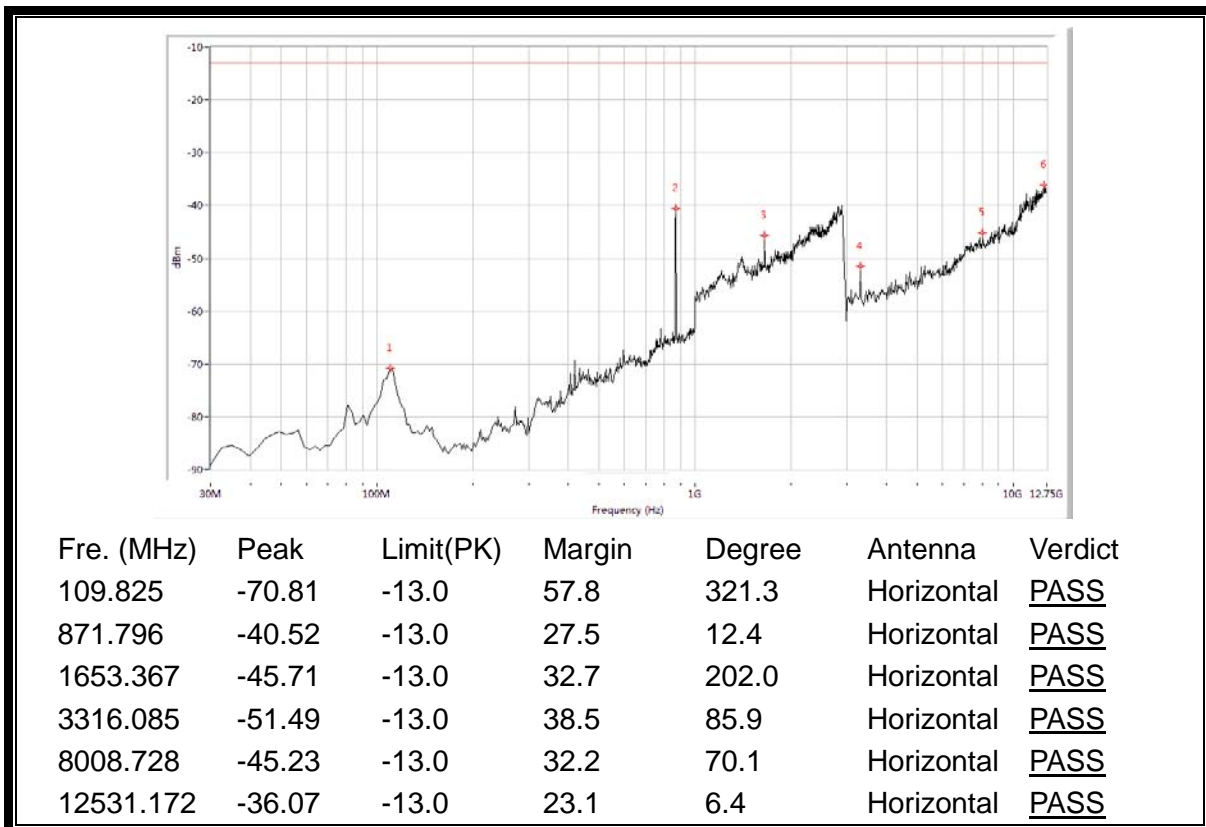
(Plot E.1: WCDMA 850MHz Channel = 4132, Test Antenna Horizontal)
