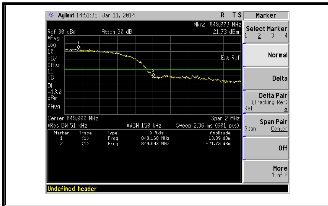
(Plot R: HSPA+ 850 Channel = 4233)
