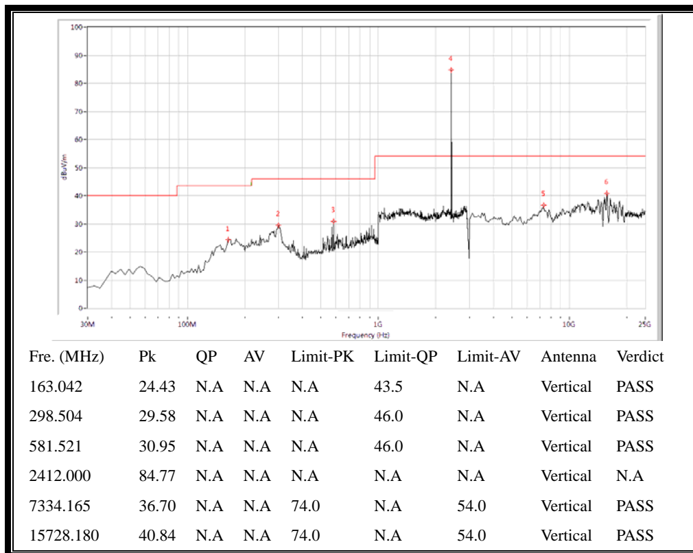
(Plot A.3: Antenna Vertical, 30MHz to 25GHz)
