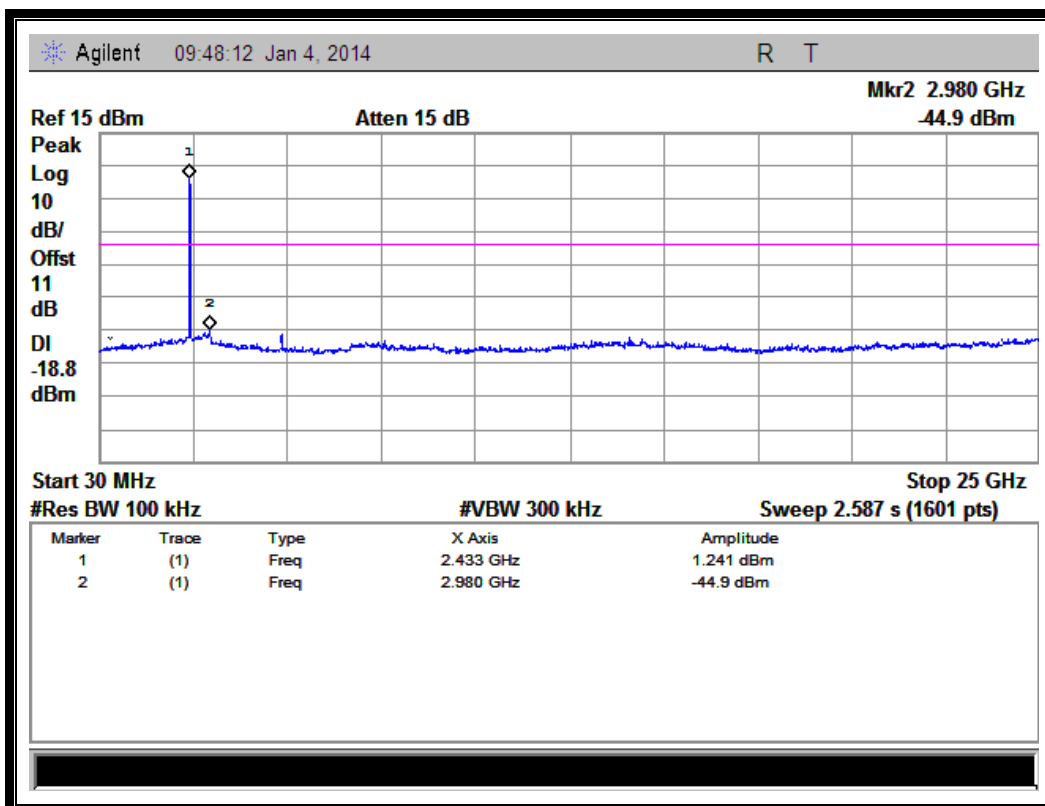
(Plot H.1: Channel = 6, 30MHz to 25GHz)
