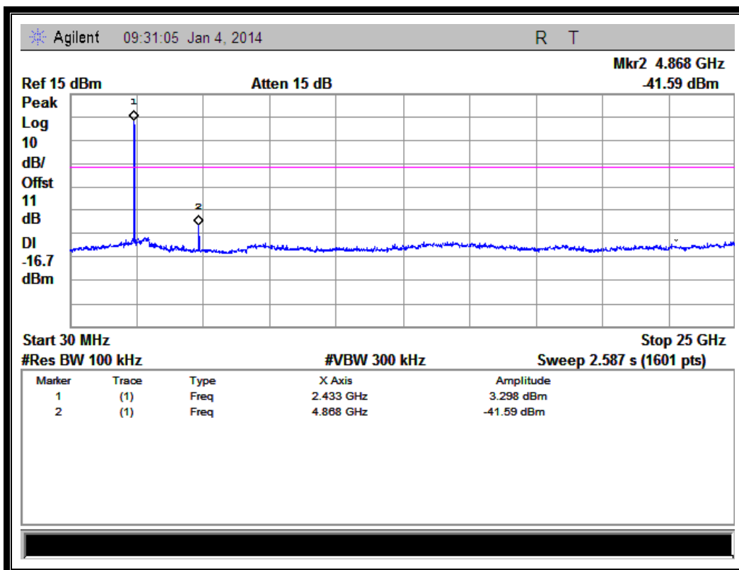
(Plot B.1: Channel = 6, 30MHz to 25GHz)
