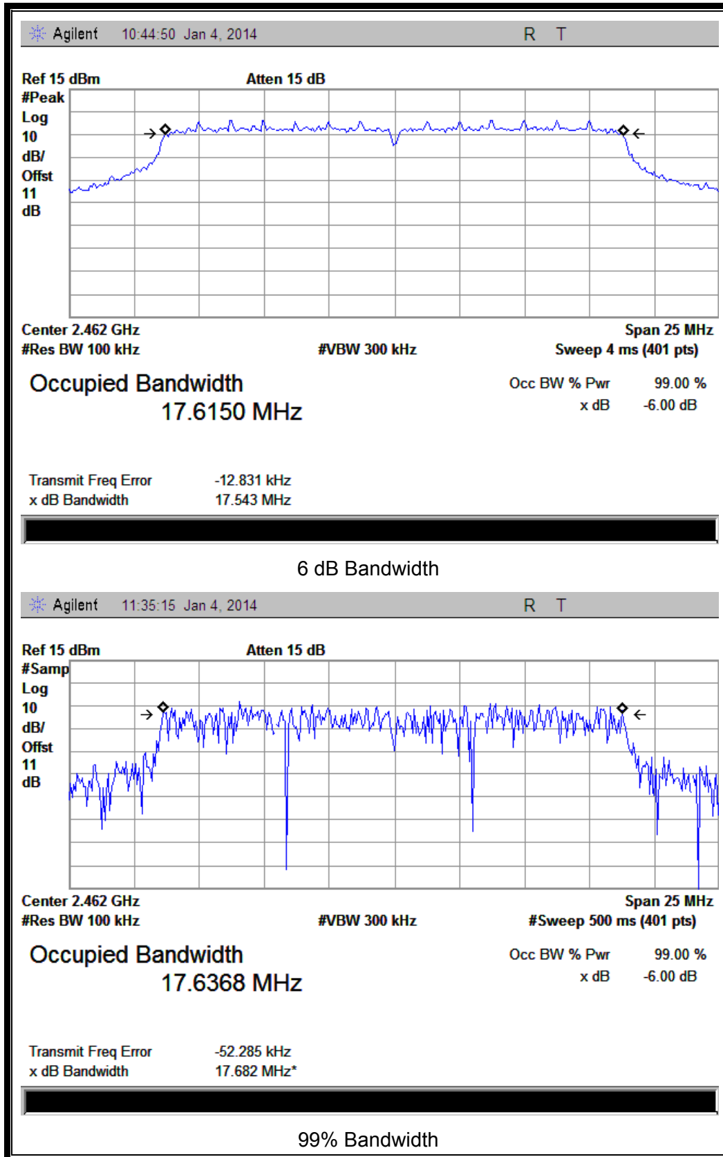
(Plot I: Channel 11: 2462MHz @ 802.11n-20)
