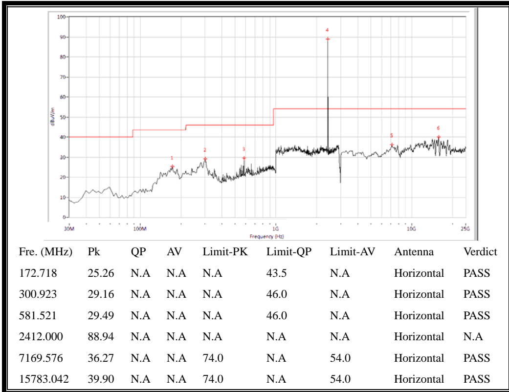
(Plot A.2: Antenna Horizontal, 30MHz to 25GHz)
