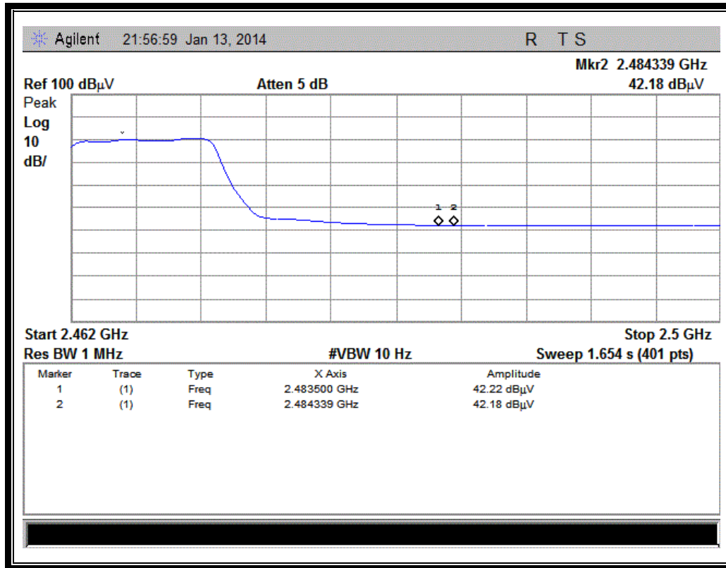
(Plot D2: Channel = 11 AVG @ 802.11g)
