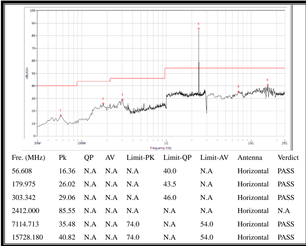
(Plot G.2: Antenna Horizontal, 30MHz to 25GHz)
