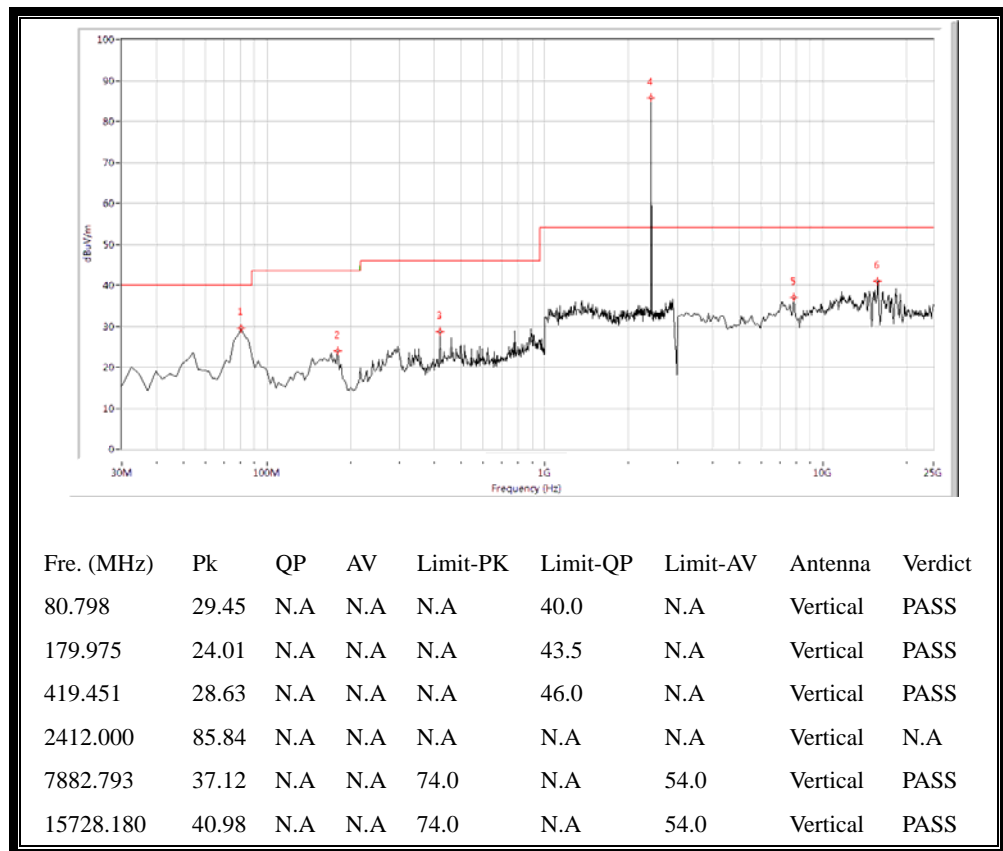
(Plot G.3: Antenna Vertical, 30MHz to 25GHz)
