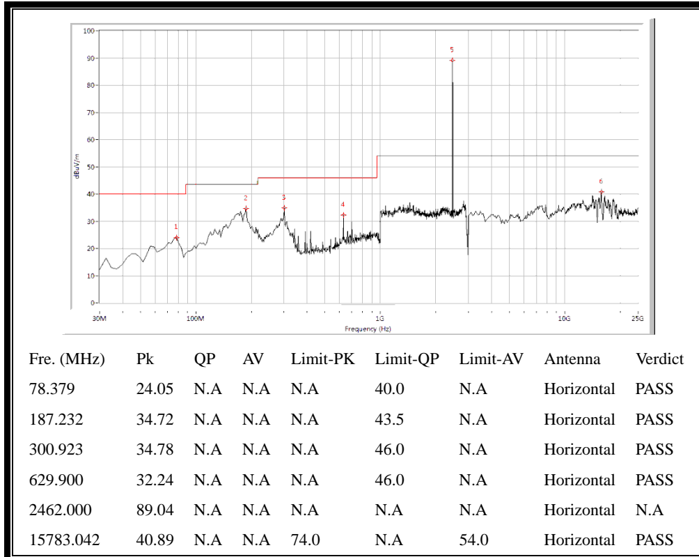
(Plot F.2: Antenna Horizontal, 30MHz to 25GHz)
