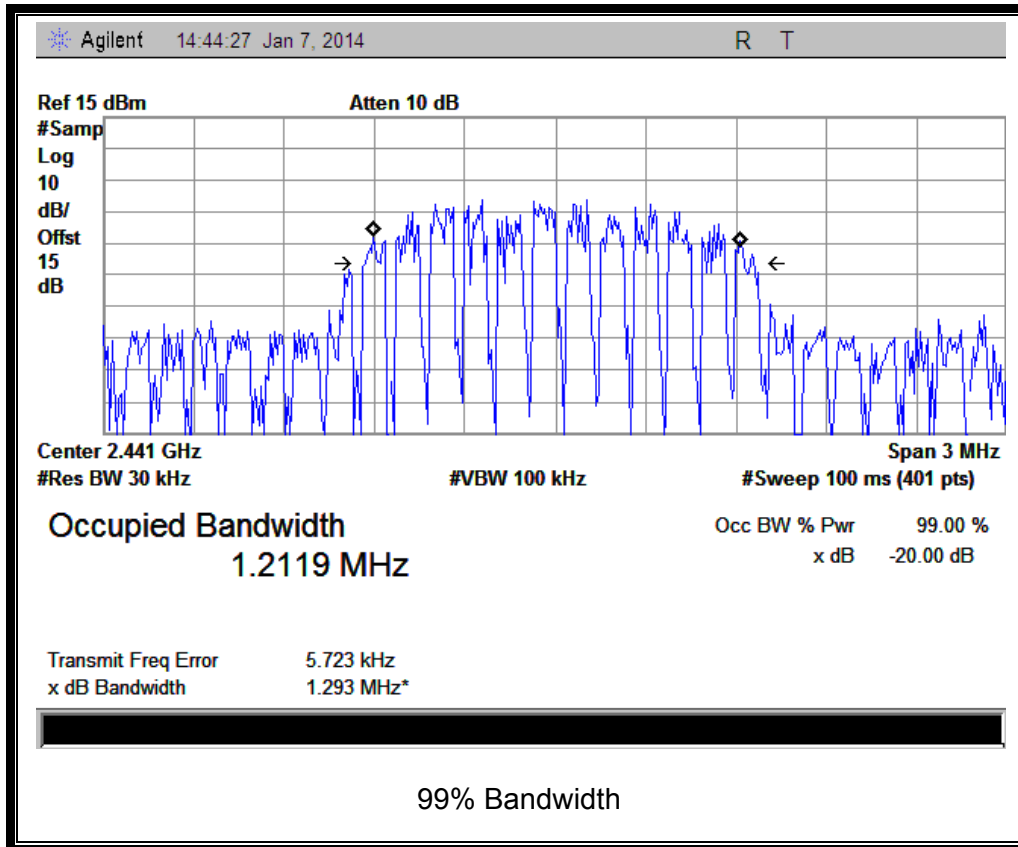
(Plot H: Channel = 2441 @ 8-DPSK)
