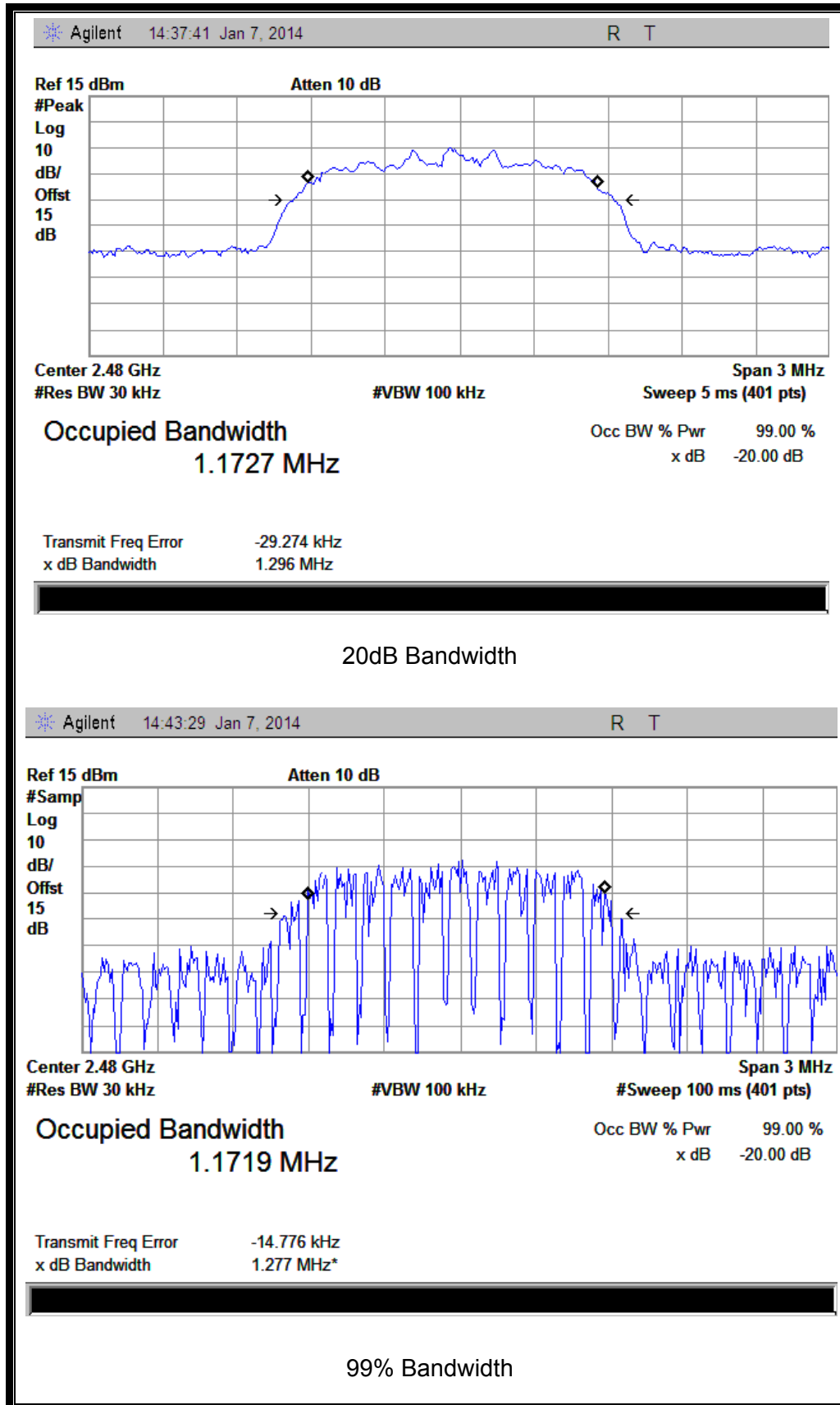
(Plot F: Channel = 2480 @ \pi/4 -DQPSK)
