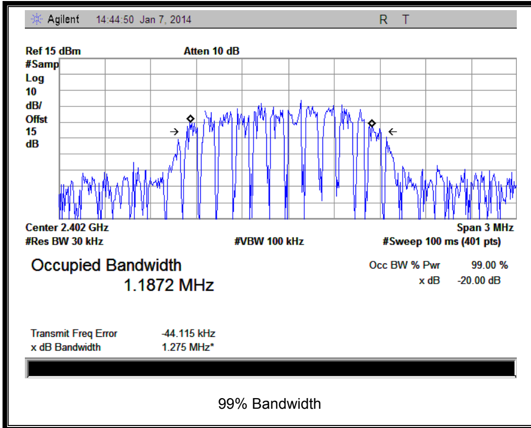
(Plot G: Channel = 2402 @ 8-DPSK)
