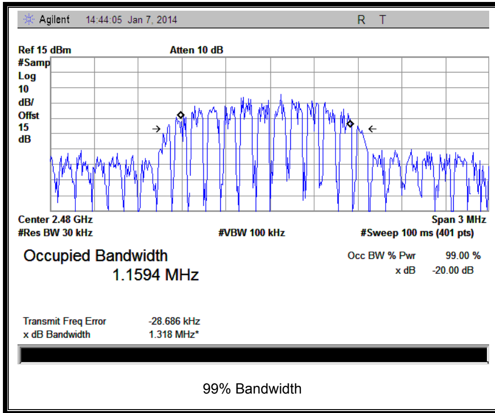
(Plot I: Channel = 2480 @ 8-DPSK)
