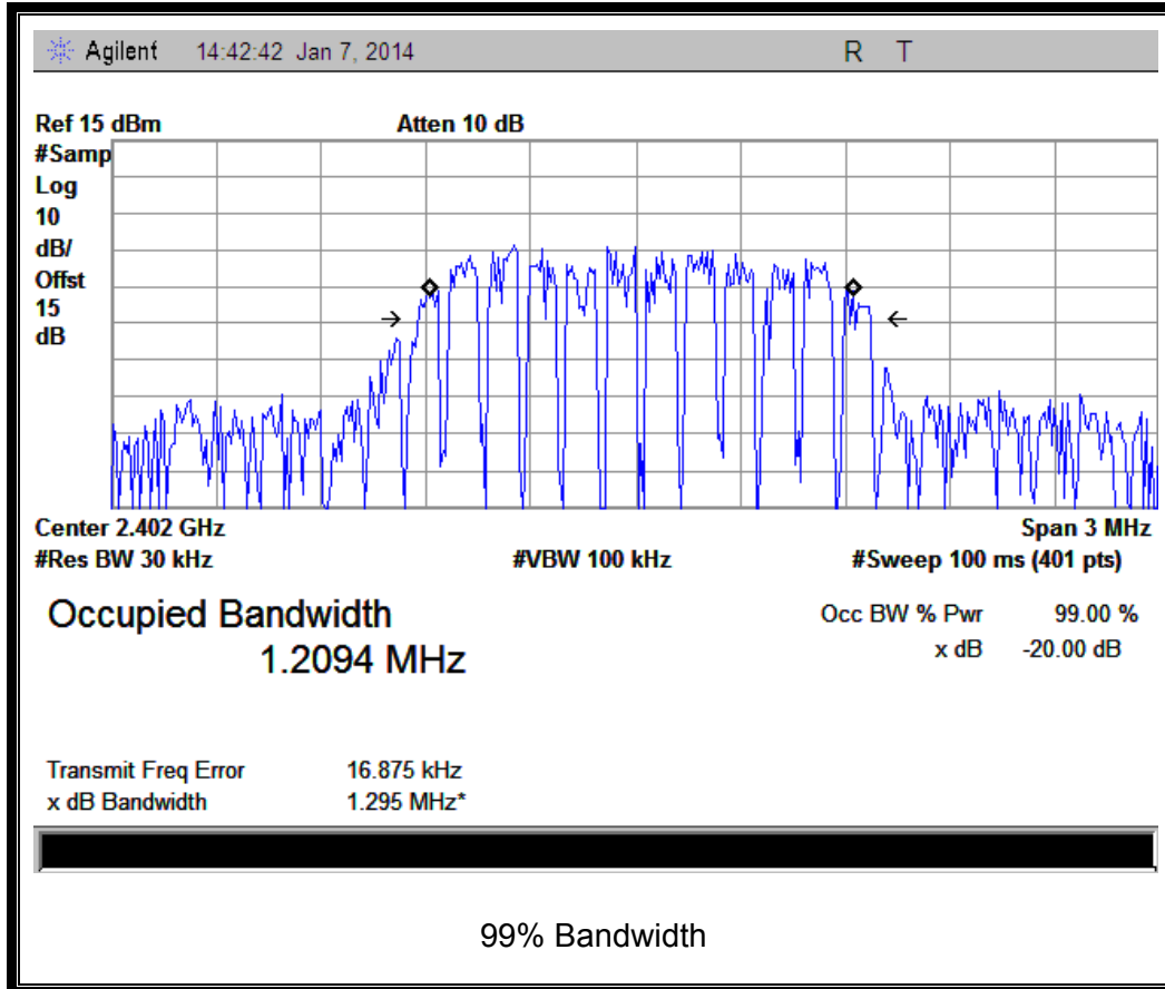
(Plot D: Channel = 2402 @ \pi/4 -DQPSK)
