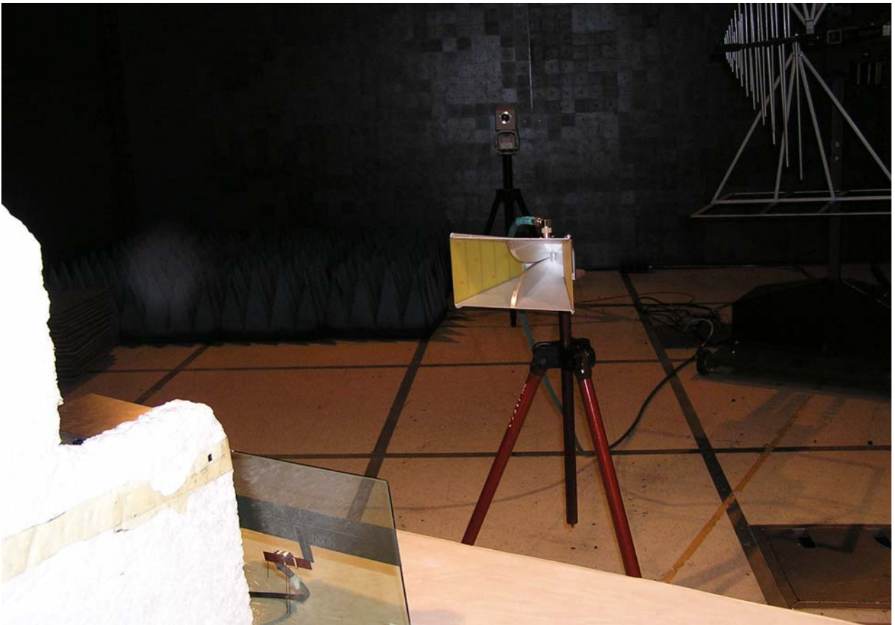
RADIATED EMISSIONS - Back
