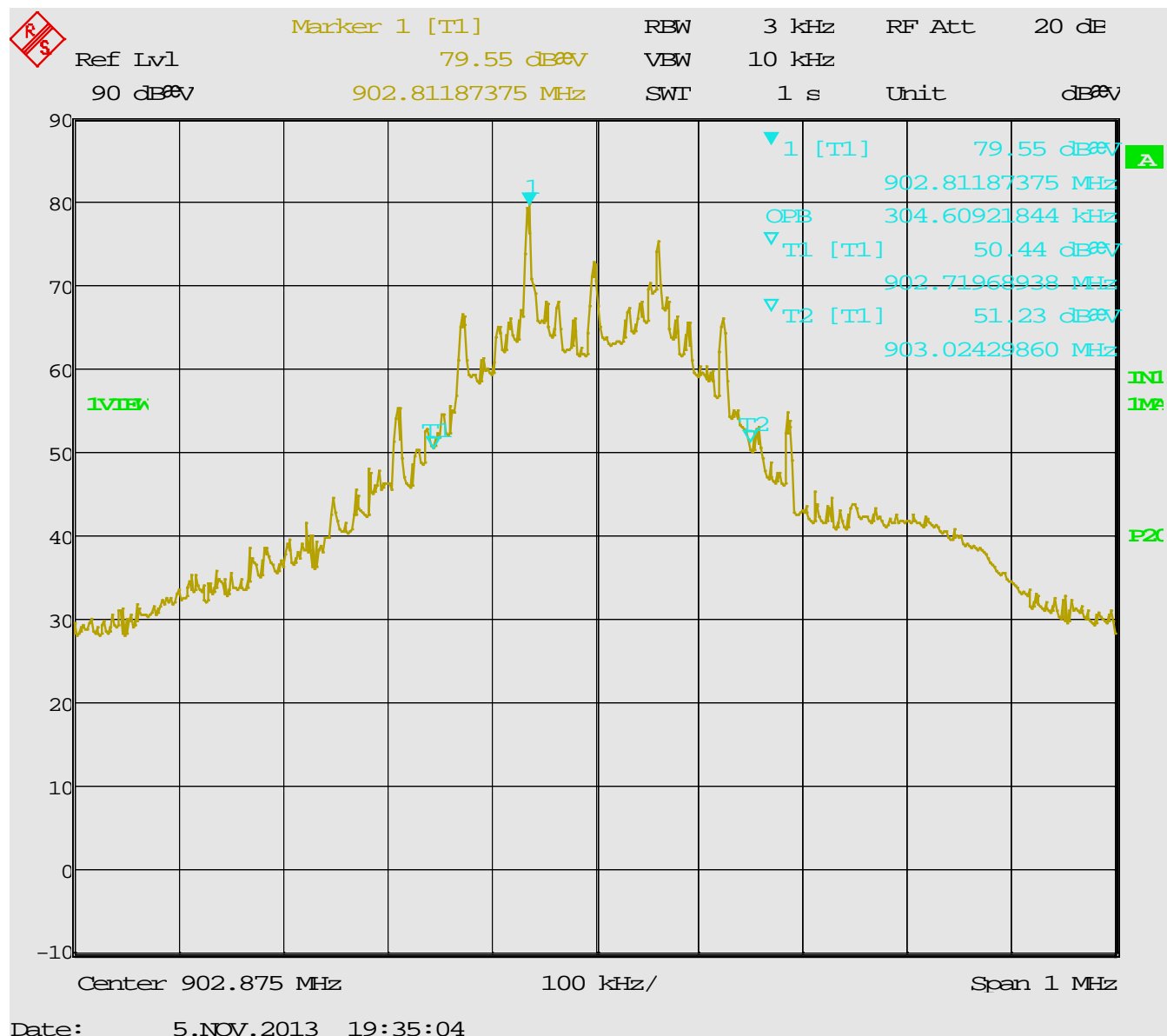
Figure 3 – 99% Power Bandwidth = 305 kHz
