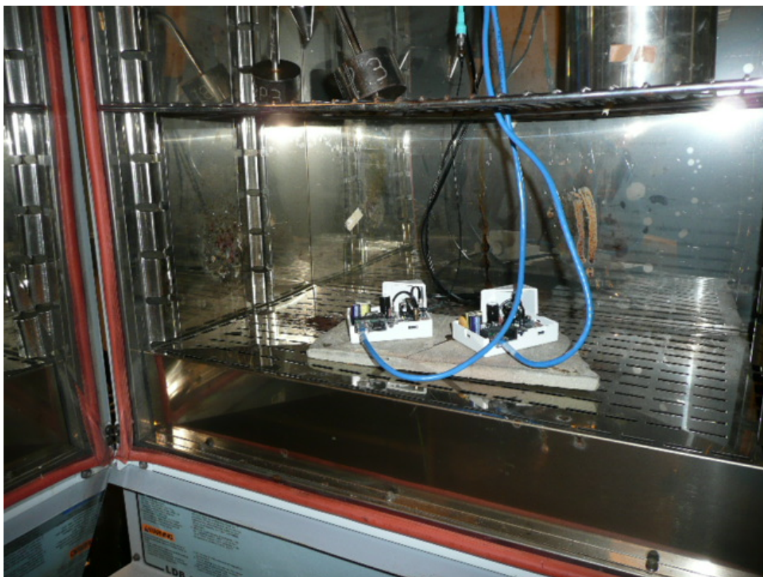
Figure 4 – Temperature and Frequency Stability Measurement
