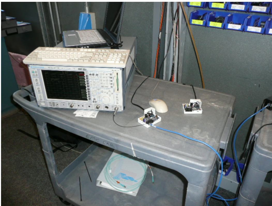
Figure 1 – Output Power and Bandwidth Measurements
